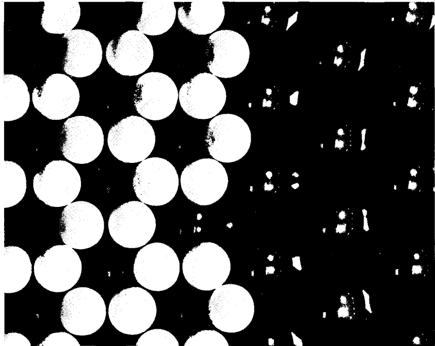
At Cornell, J. M. Blakely has measured the degree of segregation and atomic arrangement of carbon atoms on nickel surfaces. He has identified three states of different carbon coverage as a function of temperature: G as bulk graphite on nickel surface; B as one atomic layer of carbon on nickel; and A as isolated carbon atoms on nickel. A photograph of a ball model depicts, on the left-hand portion, the probable arrangement of one atomic layer of carbon. [Photo by J. M. Blakely]
