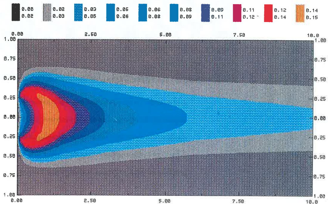
Model flame. In this supercomputer-generated image, the hottest sections of a flame have the hottest colors.
