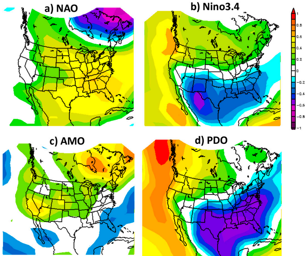
FIG. 8. Spatial linear correlation map between the SAT and DJFM indices of (a) NAO, (b) Niño-3.4, (c) AMO, and (d) PDO during 1949–2016.
