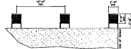
3 GROUND PLANE APPROACH MARKERS SCALE: NONE
