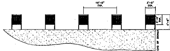
2 THRESHOLD MARKERS SCALE: NONE (ENDS OF BOTH SRWAYS)
