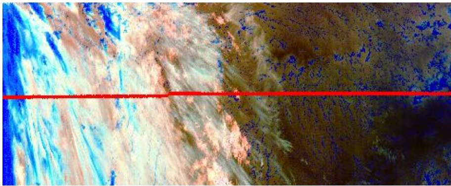
Figure 2 A false color image constructed from 11 – 12 \mu\text{m} BT (Red), 4 – 11 \mu\text{m} BT (Green) and 11 \mu\text{m} BT reversed (Blue). Data are taken from AQUA/MODIS and CALIPSO/CALIOP on August 10, 2006 from 20:35 to 20:40 UTC. The red line is the CALIPSO track. In this color combination, cirrus clouds appear white but as the optical thickness increases, the ice clouds appear as light blue/cyan. Low-level water clouds appear as dark blue, and mid-level water clouds tend to have a red/orange color.
