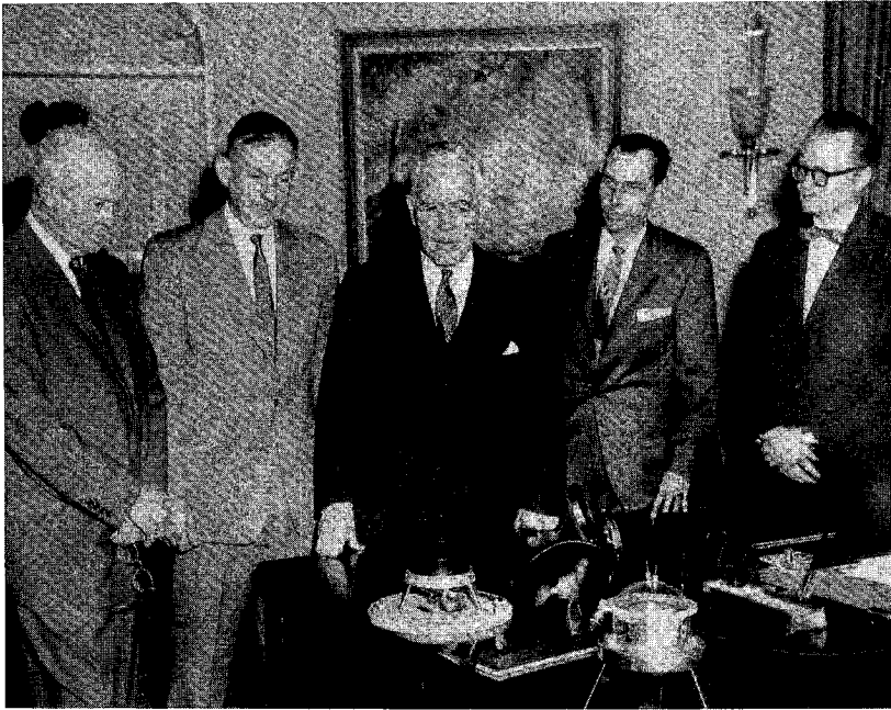
AEC Chairman John McCone describes the SNAP-3 device to President Eisenhower as it sits on his desk in the Oval Office of the White House, January 16, 1959. The small light-weight device is a radioisotope-fueled thermoelectric generator for use in space missions. Left to right: President Eisenhower, Major General Donald J. Keirn, assistant director for aircraft reactors (AEC), Chairman McCone, Colonel Jack Armstrong, deputy assistant director for aircraft reactors (AEC), and Lt. Colonel Guveren M. Anderson, project officer, missile projects branch, division of reactor development (AEC).
