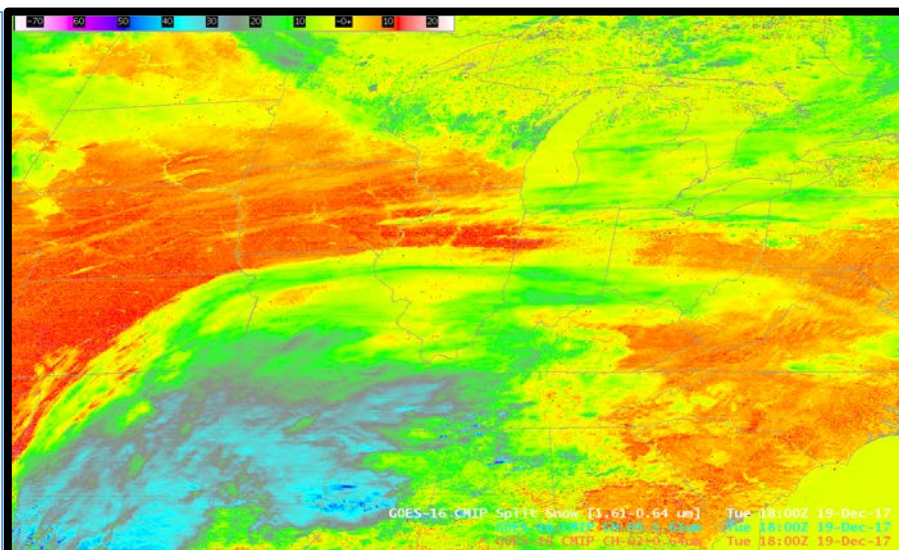
Split Snow Channel Difference from GOES-16 ABI, 1800 UTC 19 December 2017
