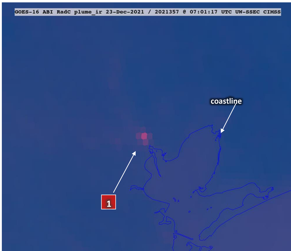
Plume from GOES-16 ABI at 0701 UTC, 23 December 2021.
