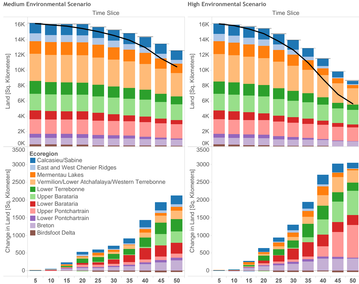
Figure 75: Land Outcomes (bars) and Future Without Action (black line) over Time by Ecoregion for 2017 Draft Coastal Master Plan under Medium Environmental Scenario (left) and High Environmental Scenario (right).
