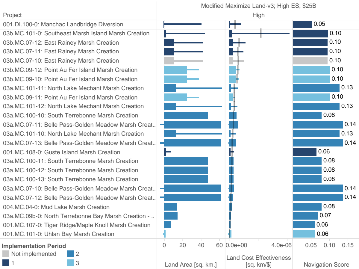
Figure 60: Sediment Diversion and Marsh Creation Projects with High Navigation Scores (>= 0.05) Ordered by Land Cost-Effectiveness and Colored by Implementation in the Modified Maximize Land Alternative.
