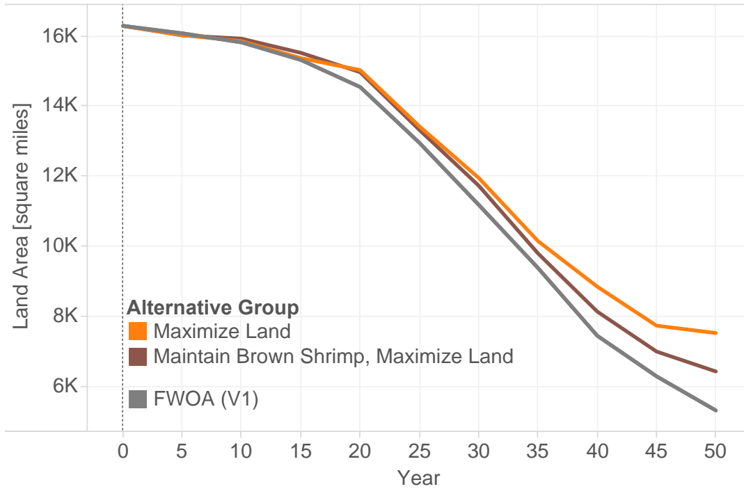
Figure 57: Land over Time under High Environmental Scenario for Future Without Action (gray line), Maximize Land (orange line), and Maintain Brown Shrimp, Maximize Land Alternatives ($25B Funding, High Environmental Scenario).
