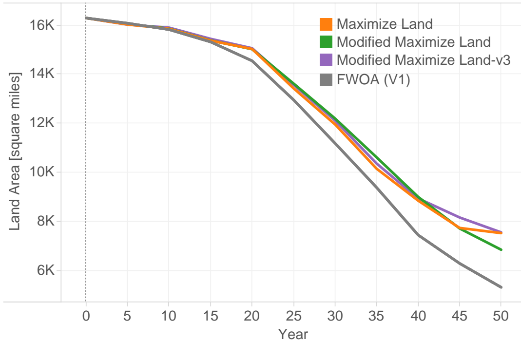
Figure 53: Land over Time under the High Environmental Scenario for Future Without Action, Maximize Land and Modified Maximize Land Alternatives ($25B Funding, High Environmental Scenario).
