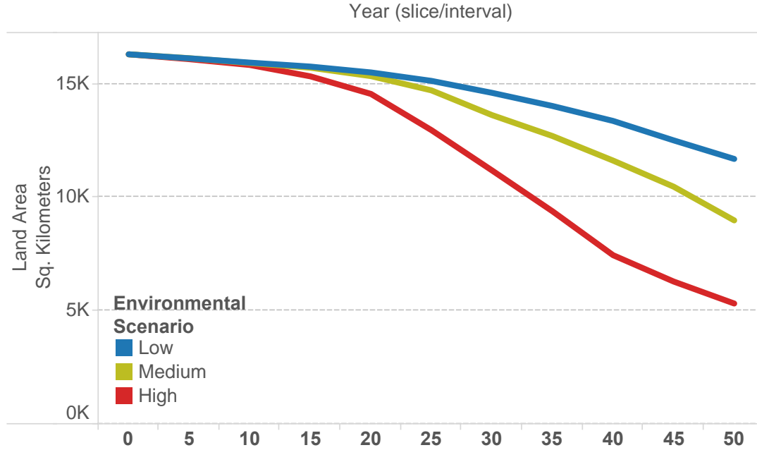
Figure 20: Coast Wide Change in Future Without Action Land Area for Three Environmental Scenarios.
