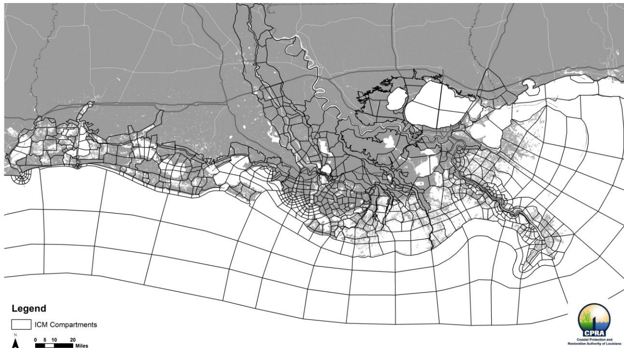
Figure 1: Hydrology Compartments within the Integrated Compartment Model.
