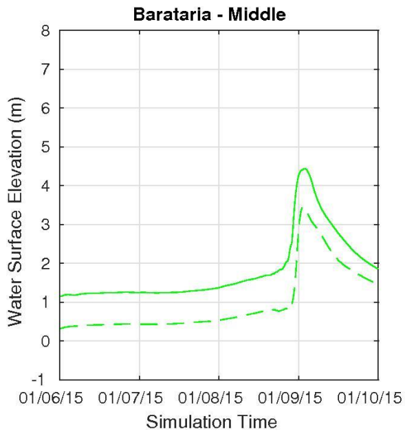
Figure 32: Example QA/QC Image Showing the Time Series of Water Surface Elevation at Three Locations in Barataria Bay and the Comparison to Initial Conditions.
