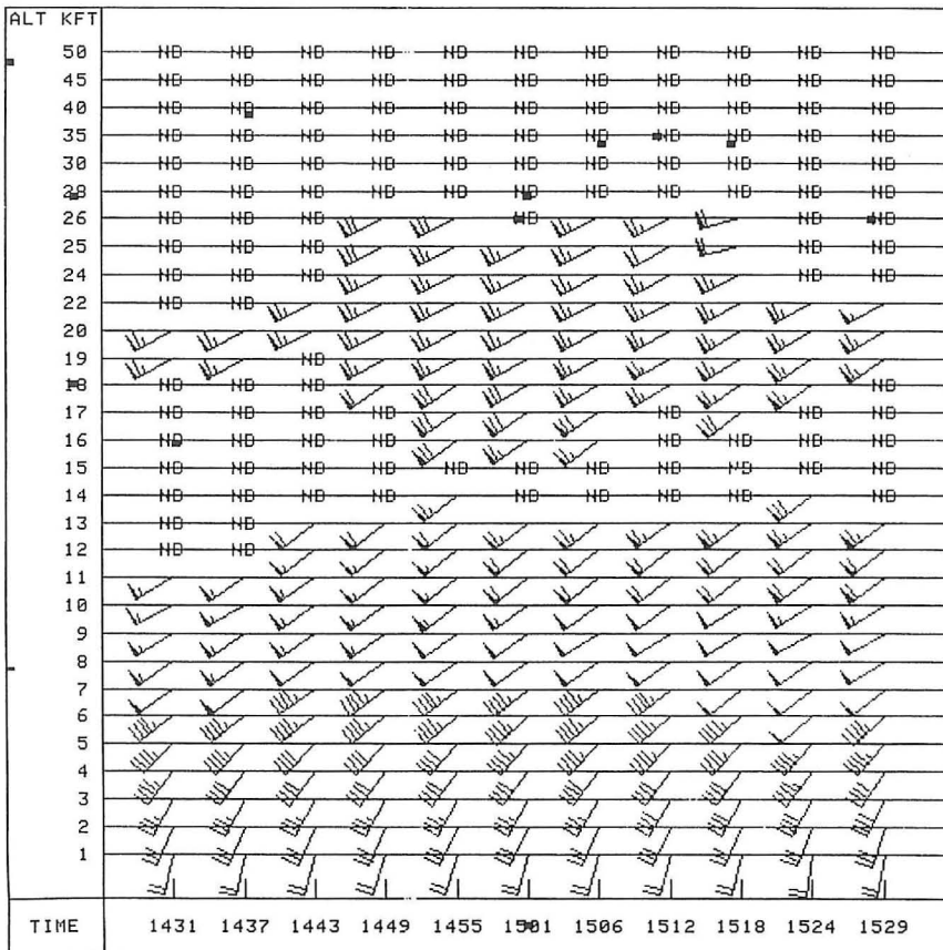
Fig. 22. Time series (UTC) of the VAD Wind Profile (VWP) product from the Maxwell Air Force Base, Alabama WSR-88D (KMXF). Wind bars and flags are the same as in Fig. 11.
