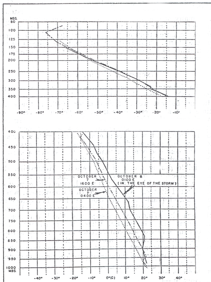
FIGURE 2.—Soundings made at Tampa during the approach and passage of the hurricane.
