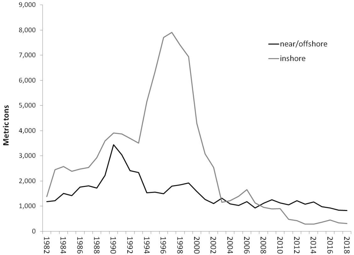
Figure 65. Commercial lobster landings in the Southern New England stock unit 1982 to 2018 from inshore (SA 538, 539, 611; grey) and offshore/nearshore (SA 537, 612, 613, 614, 615, 616; black) regions.
