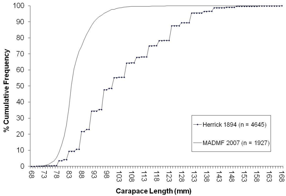
Figure 59. Comparison of cumulative length distribution of egg-bearing female lobsters from Buzzards Bay, MA (2007)/Cox Ledge, MA (1894).
