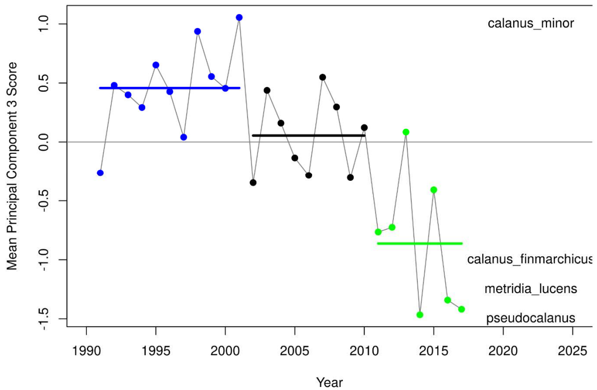
Figure 51. Yearly mean values of zooplankton community third principal component from NEFSC Fall EcoMon plankton surveys. Colors indicate different candidate regimes with horizontal lines indicating mean values during the regime. High PCA scores are associated high densities of C. minor with low scores associated with high densities of C. finmarchicus , M. lucens and Pseudocalanus .
