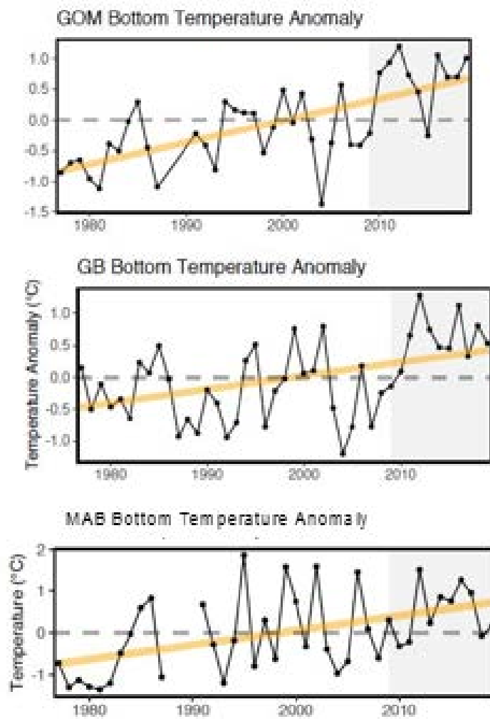
Figure 23. Mid-Atlantic Bight (MAB), Georges Bank (GB), and Gulf of Maine (GOM) bottom temperature anomalies. Yellow line indicates significant increasing trend at p < 0.05 . (Source: Gaichas et al., 2020A and Gaichas et al., 2020B).
