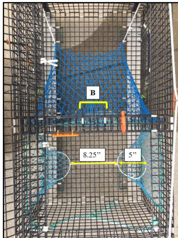
Figure RIDEM 2. General trap configurations for a RI VTS trap. 'B' signifies where the bait is strung and hung into the kitchen. Dimensions lengths are in inches.
