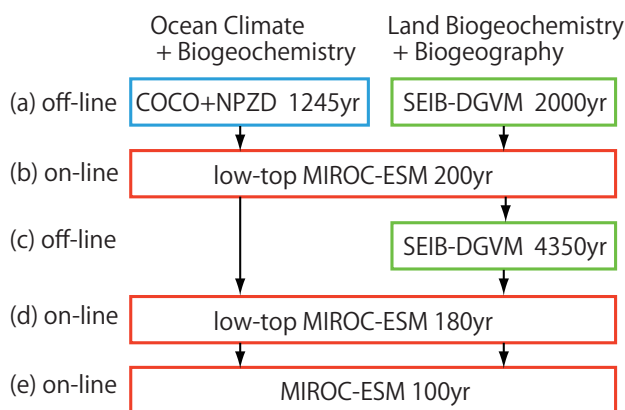
Fig. 3. Spin-up procedures of MIROC-ESM.
