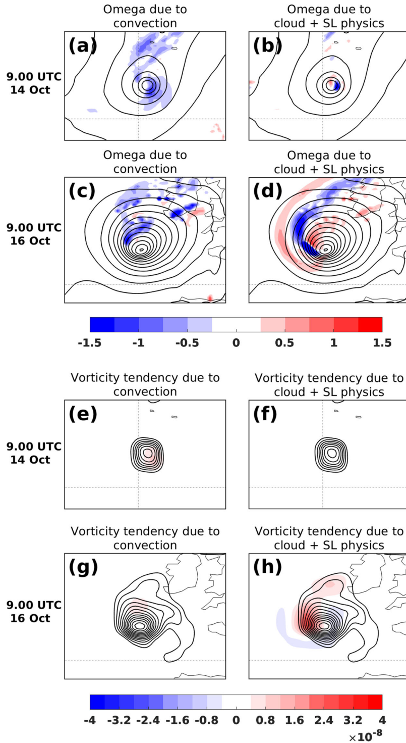
Fig. 16. Panels (a) – (d) show vertical motion (shading, Pa s -1 ) at 700 hPa and sea level pressure (contours, with 4-hPa interval), and panels (e) – (h) show vorticity tendency (shading, s -2 ) and relative vorticity (contours, starting from 5 \times 10^{-5} s -1 , with 5 \times 10^{-5} s -1 interval) averaged over the 900–800-hPa layer. The left-hand panels [(a), (c), (e), and (g)] show vertical motion and vorticity tendency due to the convection parametrization, and the right-hand panels [(b), (d), (f) and (h)] show vertical motion and vorticity tendency due to the microphysics parametrization. The upper panels in both vertical motion [(a) and (b)] and in vorticity tendency [(e) and (f)] show the situation at 9 UTC 14 October (tropical phase), and the lower panels [(c), (d), (g) and (h)] at 9 UTC 16 October (extratropical phase). The size of the panels is 16° longitude by 12° latitude, centred on the cyclone vorticity maximum.
