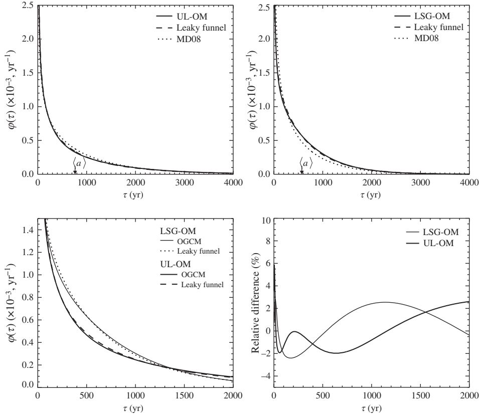
Fig. 2. Global water age distribution \varphi (solid line) versus age in two 3-D OGCMs, UL-OM (top left) and LSG-OM (top right), compared to that predicted by the leaky funnel (dashed line). The leaky funnel curve in each panel is obtained with the parameters appropriate to the corresponding OGCM from Table 1. In the two upper panels, the curve computed with the parameters as estimated by the method of MD08 is also represented (dotted line). The arrow in those two panels points to the actual global mean water age \langle a \rangle obtained with each OGCM. The lower two panels allow the comparison of both OGCMs with focus on ages under 2000 years. Global water age distribution \varphi (bottom left) as obtained with LSG-OM (thin solid) and UL-OM (thick solid) and as estimated by the leaky funnel for each OGCM: LSG-OM (dotted) and UL-OM (dashed). Relative difference (bottom right) between the OGCM and the leaky funnel global water age distributions for LSG-OM (thin solid) and UL-OM (thick solid).
