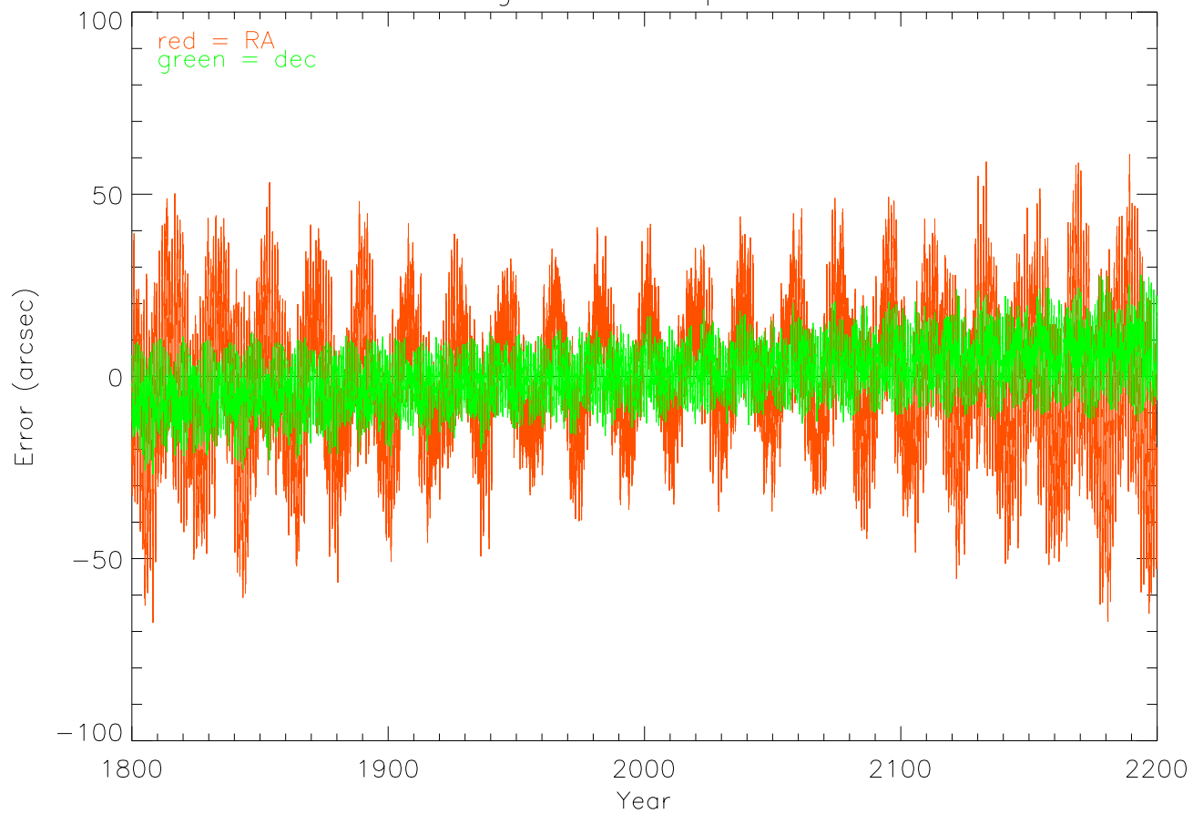
Error in Sun Algorithm in Equatorial Coordinates
