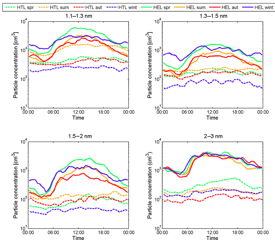
Figure 6. The median diurnal variation in particle concentration in four size bins (1.1–1.3, 1.3–1.5, 1.5–2, and 2–3 nm) in Hyytiälä (HTL; dashed lines) in 2011 and in Helsinki (HEL; solid lines) in 2015. The data are divided into different seasons: spring (spr), summer (sum), autumn (aut), and winter (wint).
