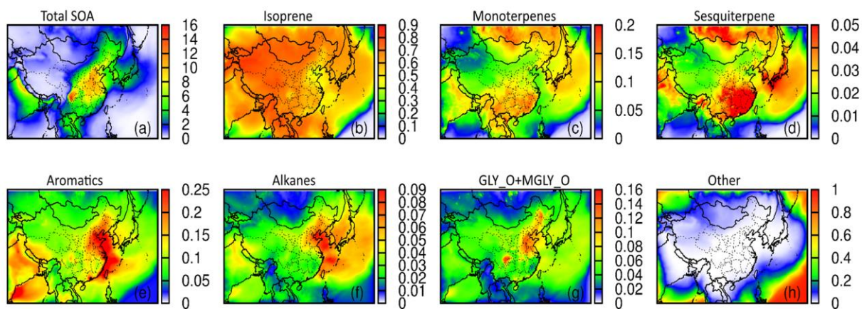
Figure S5 Predicted average SOA concentrations in summer 2013 and relative contributions of different precursors to total SOA.
