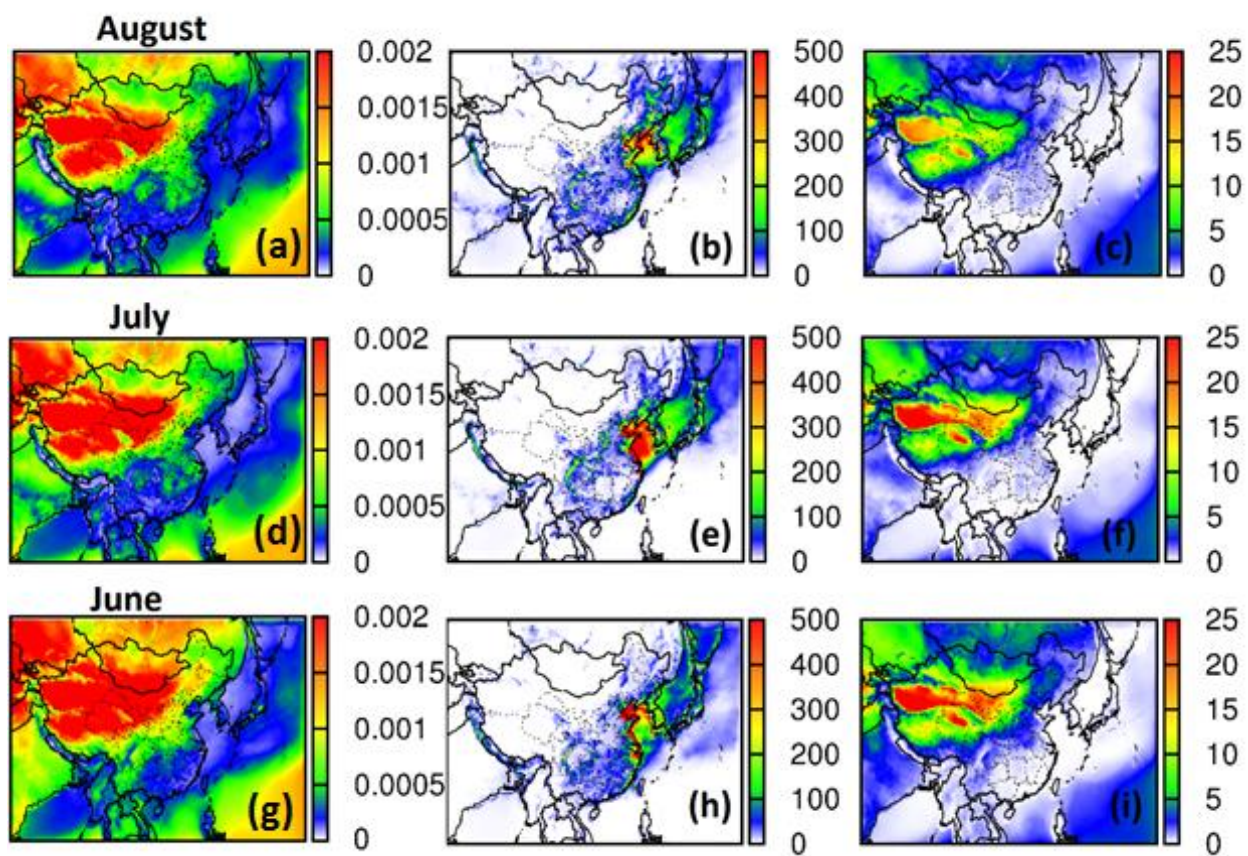
Figure S1 Summertime (a,d,g) uptake coefficients for isoprene epoxides; (b,e,h) aerosol water content ( \mu\text{g m}^{-3} ) and (c,f,i) molality of H + ( \text{mol kg}^{-1} water).
