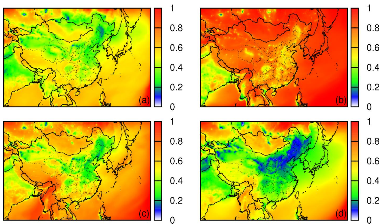
Figure S3 Fractional contributions of predicted SOA to total OA (SOA+POA) for (a) spring, (b) summer, (c) autumn, and (d) winter 2013
