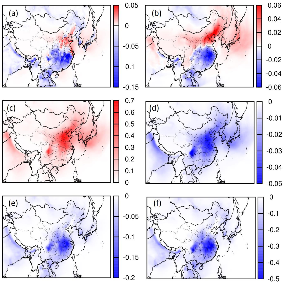
Figure S8 Predicted changes spatial distribution of August isoprene SOA components (a) semi-volatile, (b) oligomers, (c) IEPOX, (d) MAE, (e) GLY and (f) MGLY due to reduction of NOx emission by 50%. (sensitivity case – base case, units are \mu\text{g m}^{-3} ).
