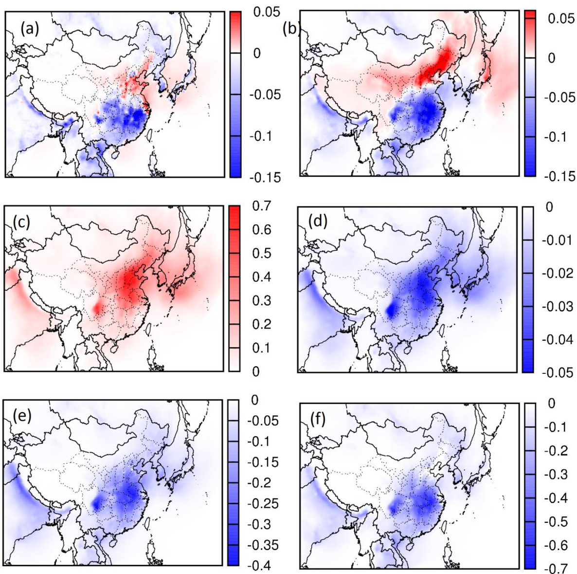
Figure S7 Predicted changes in the spatial distribution of August SOA components (a) semi-volatile, (b) oligomers, (c) IEPOX, (d) MAE, (e) GLY and (f) MGLY due to reduction of NO x emission by 50%. (sensitivity case – base case, units are \mu\text{g m}^{-3} ).
