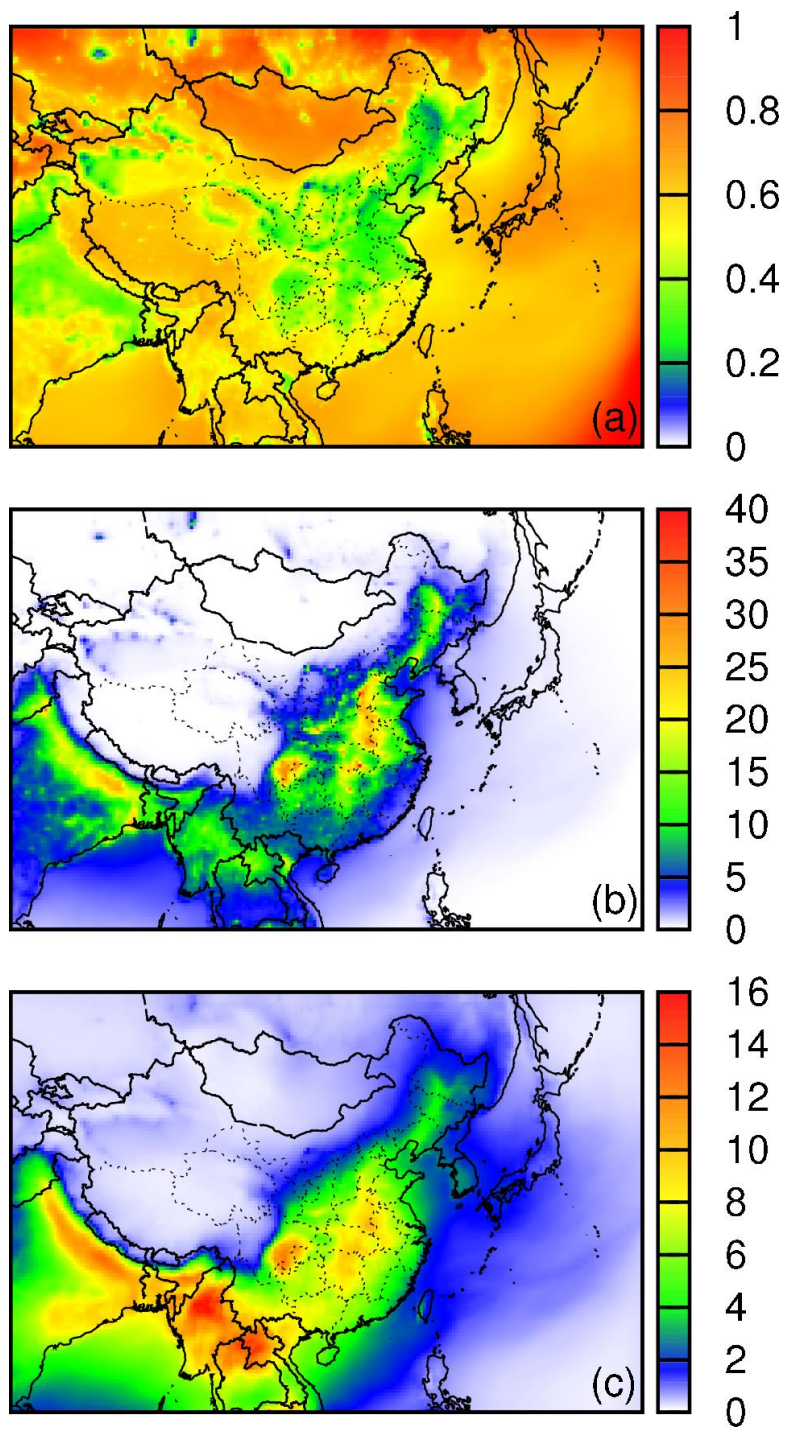
Figure S4 (a) Fractional contributions of predicted annual average SOA to total OA (SOA+POA), (b) annual average POA and (c) annual average SOA. Units are \mu\text{g m}^{-3} .
