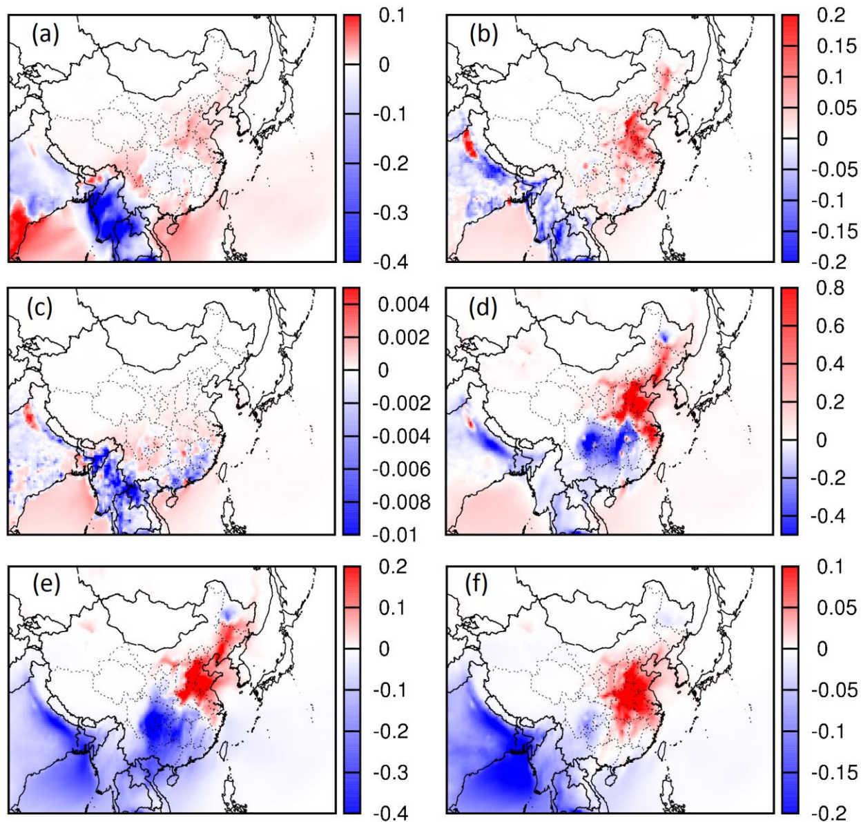
Figure S9 Predicted changes in spatial distribution of January SOA from different precursors, (a) ISOP, (b) TERP, (c) SESQ, (d) ARO1+ARO2, (e) ALK5, and (f) primary GLY+MGLY
