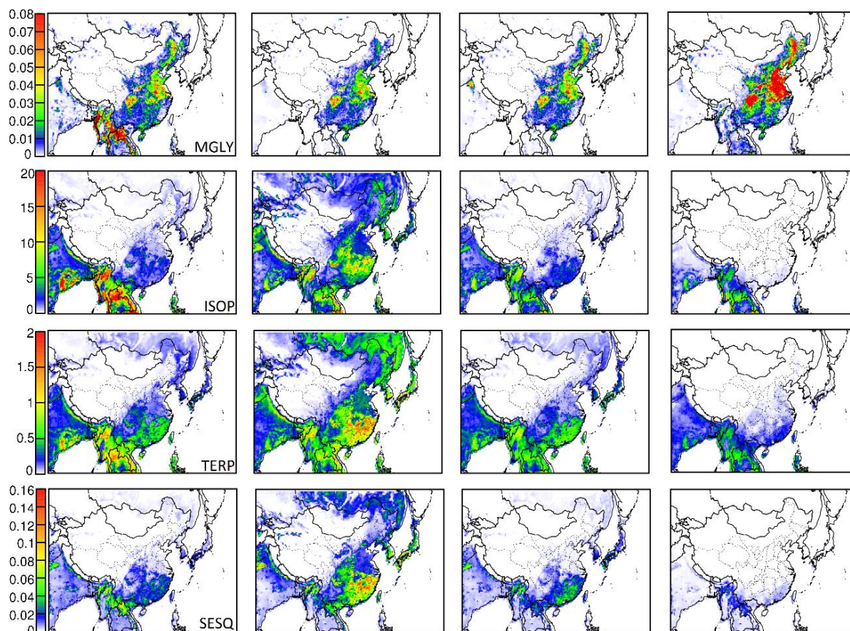
Figure S2 (continue) Seasonal average of SOA precursor emission (MGLY, ISOP, TERP and SESQ) in (a) spring, (b) summer, (c) autumn, and (d) winter 2013. Units are moles s^{-1} .
