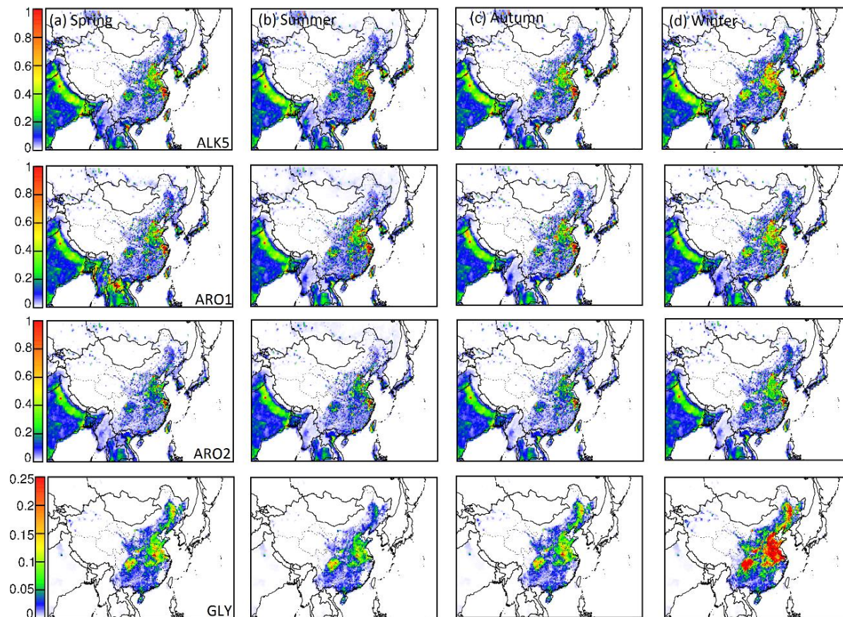
Figure S2 Seasonal average of SOA precursor emission (ALK5, ARO1, ARO2 and GLY) in (a) spring, (b) summer, (c) autumn, and (d) winter 2013. Units are moles s^{-1} .
