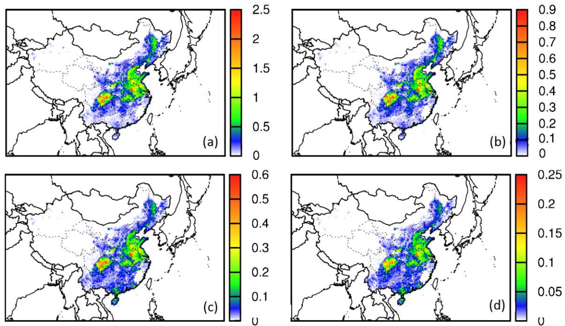
Figure S6 Monthly average emissions of GLY (a,c) and MGLY (b,d) in January and August, 2013.
