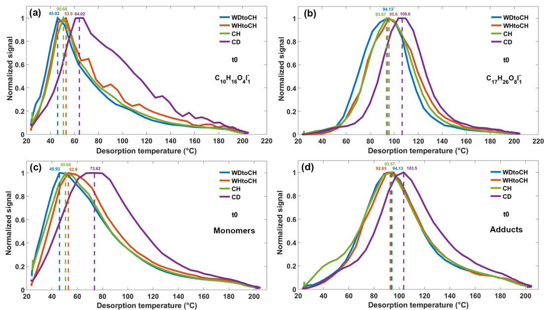
Figure 6. Thermograms of monomer C_{10}H_{16}O_4 (a) and adduct C_{17}H_{26}O_8 (b), both clustered with I_1^- at t_0 , and sum thermograms of monomers (c) and adducts (d) at t_0 . Dashed lines refer to the corresponding T_{max} .
