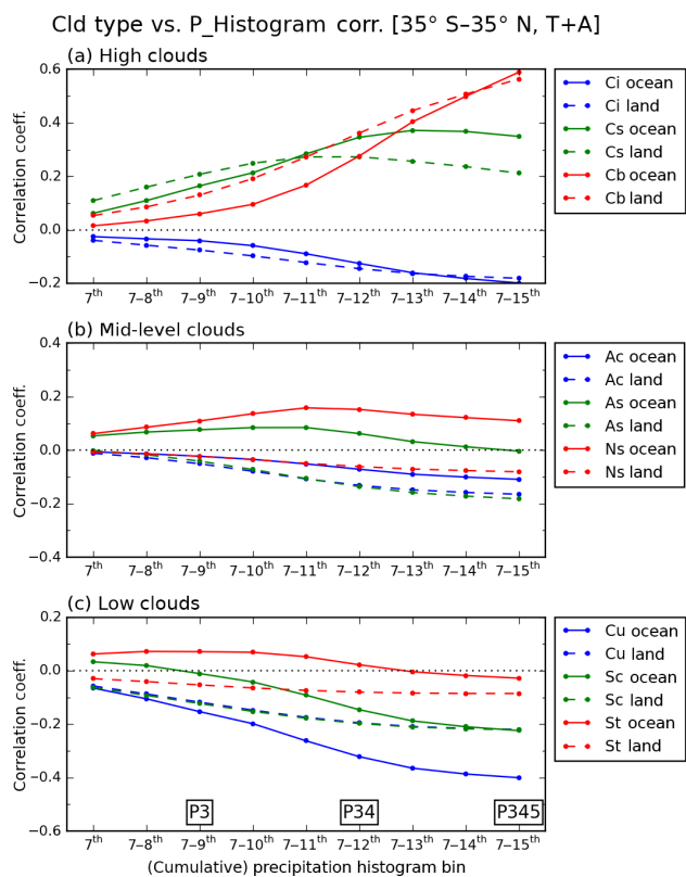
Figure 11. Correlation coefficients between cloud type CF and precipitation histogram values, for (a) high clouds ( Ci , Cs , and Cb ), (b) mid-level clouds ( Ac , As , and Ns ), and (c) low clouds ( Cu , Sc , and St ). Precipitation histogram values are added cumulatively from the seventh bin onward, so the sum from the seventh to the ninth bin corresponds to P3, and so on. Oceanic cloud results are shown in solid lines, and continental cloud results are shown in dashed lines.
