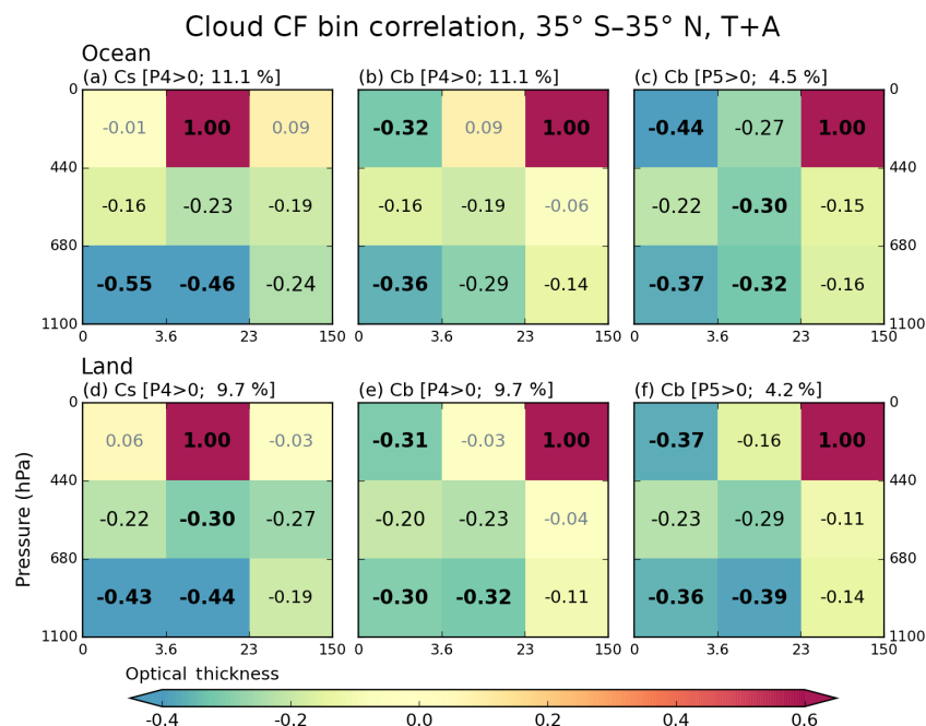
Figure 10. Conditional cross-correlation coefficients between cloud joint histogram bin CF values calculated for 13 years, based on (a) Cs CF over ocean when P_4 > 0 , (b) Cb CF over ocean when P_4 > 0 , (c) Cb CF over ocean when P_5 > 0 , (d) Cs CF over land when P_4 > 0 , (e) Cb CF over land when P_4 > 0 , and (f) Cb CF over land when P_5 > 0 . The percentage numbers above each panel are sample size ratios relative to the total number of ocean or land grid cells.
