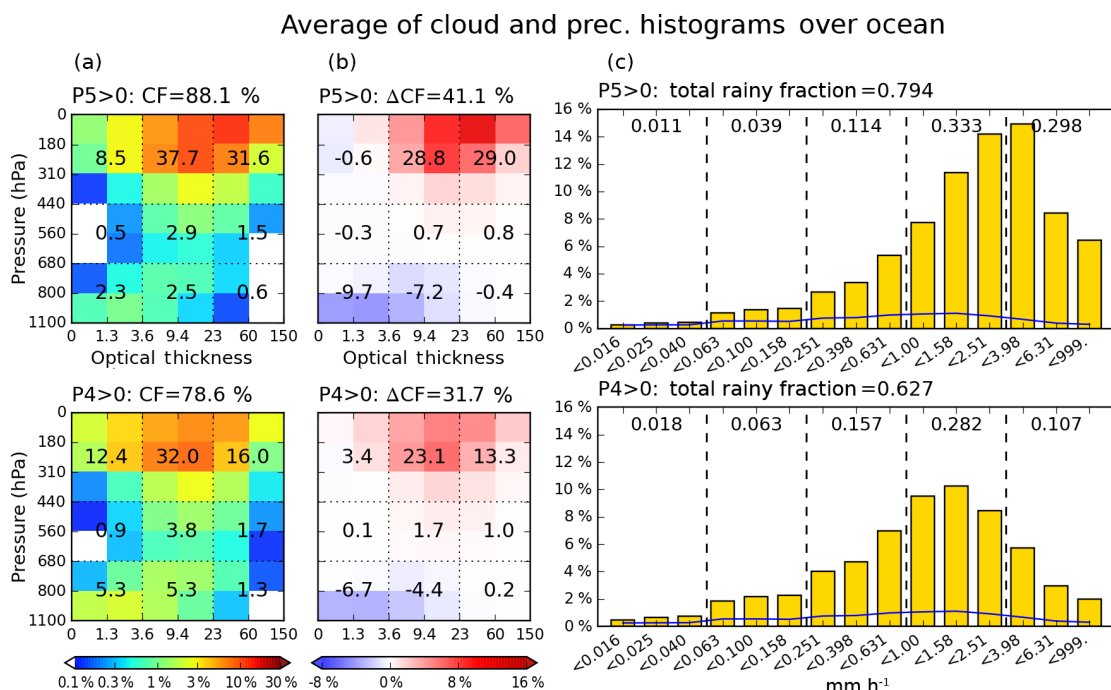
Figure 5. Conditional composite mean of 2-D joint histogram of p_c and \tau (left column), differences from overall (unconditional) mean (middle column), and precipitation histogram (right column) over the extended tropical oceans for 13 years. Top row is for P5, while bottom row is for P4 precipitation. Blue lines in precipitation histograms indicate the overall mean. Both cloud and precipitation overall means correspond to the entire domain, and not just ocean. Numbers on cloud histograms are the cloud fraction (CF; in percentage) of each cloud type, which is the sum of four or six histogram bin values assigned to the cloud type. The sum of all values is equal to the total cloud fraction provided above each panel. Numbers on precipitation histograms are the fraction of each P-group, P1 (left) to P5 (right), obtained as the sum of three individual bin values. Total rainy fraction is the sum of all P-groups' fractions (i.e., sum of 15 individual bin values).
