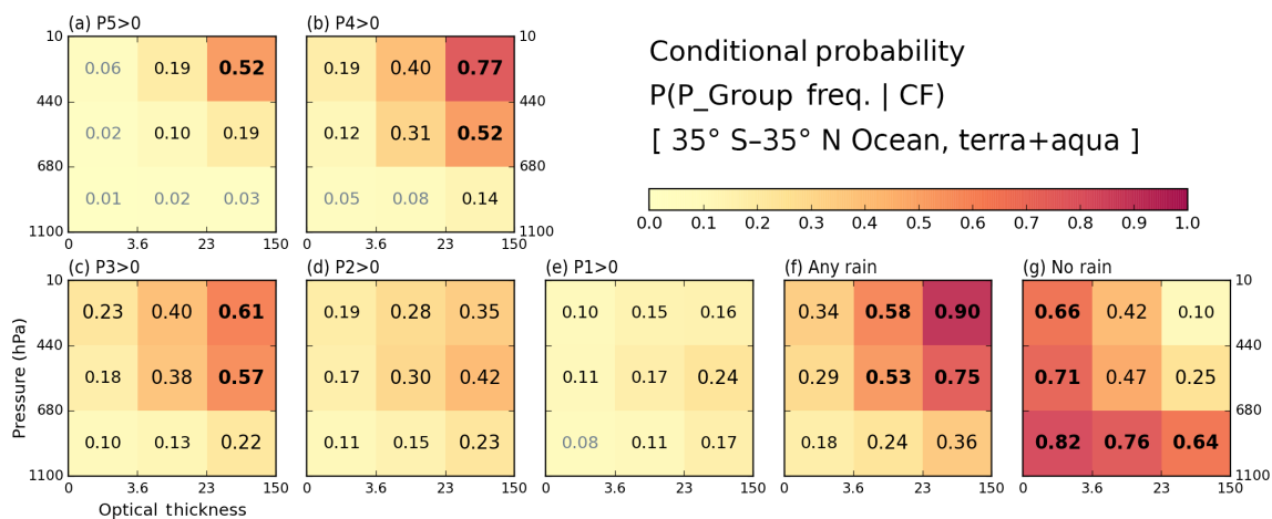
Figure 3. (a–e) Conditional probabilities of precipitation within a P-group (from TMPA) given occurrences of a cloud type (from MODIS) over ocean in the extended tropics from December 2002 to November 2015. (f) Conditional probabilities of any rain amount (sum of all P-group frequencies). (g) Conditional probabilities of no rain co-occurring with cloud. The CF threshold for cloud type occurrence is 6.25 %.
