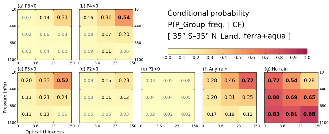
Figure 4. Same as Fig. 3, but over land.
