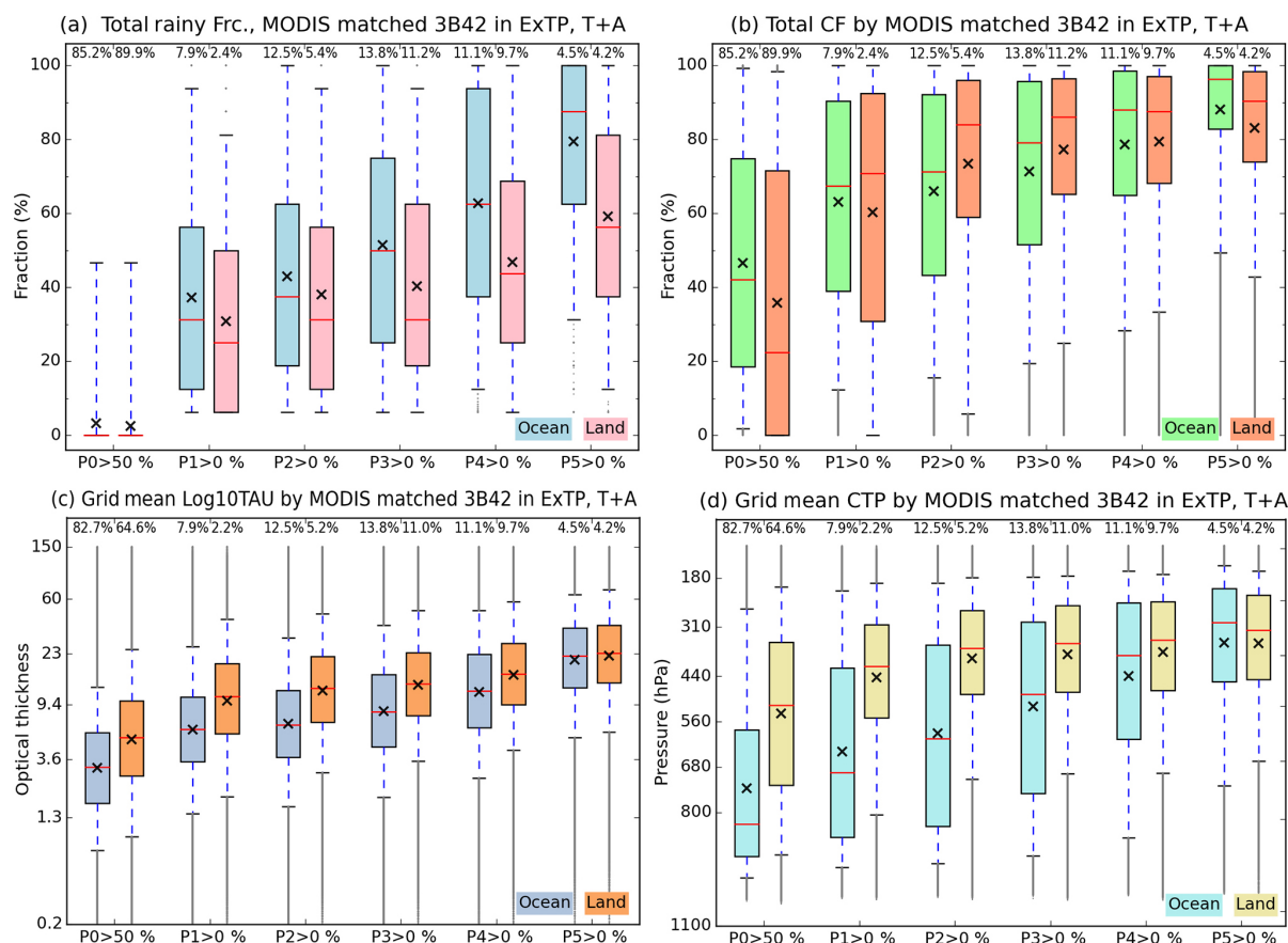
Figure 7. Box-and-whisker plot of (a) the total rainy fraction, (b) the total cloud fraction, (c) the grid-mean \log_{10}(\tau) , and (d) the grid-mean p_c conditioned by precipitation groups, separately for ocean and land. The median values are shown as red horizontal lines, and the mean values are shown as black crosses. The vertical width of the boxes indicates the interquartile range (25th–75th percentile), and the whiskers extend from 5 to 95% values. Percentage numbers above the boxes indicate the occurrence ratio of each P-group relative to the total ocean or land grid cells.
