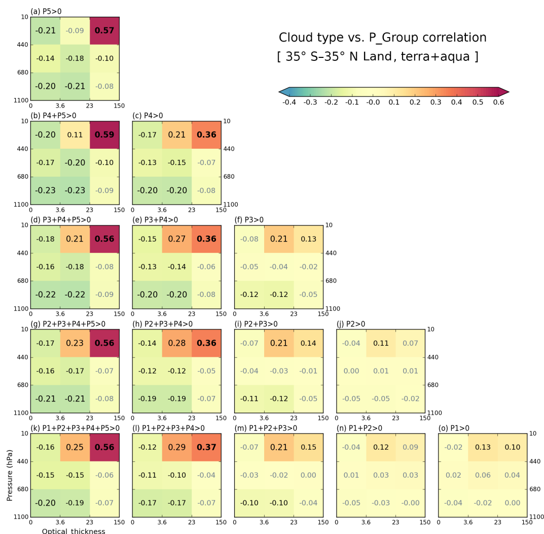
Figure 9. Same as Fig. 8, but over land.
