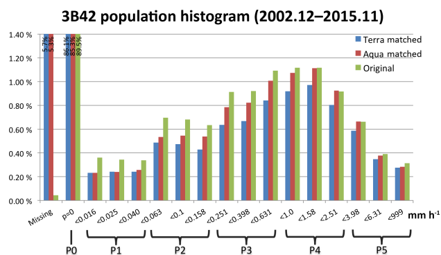
Figure 1. Histograms of TMPA original 0.25^\circ \times 0.25^\circ 3-hourly 3B42 precipitation data (green), and subsets matched with daytime Terra (blue) and Aqua (red), from December 2002 to November 2015 in the extended tropics domain. The boundaries that define the six simplified precipitation groups are shown at the bottom.
