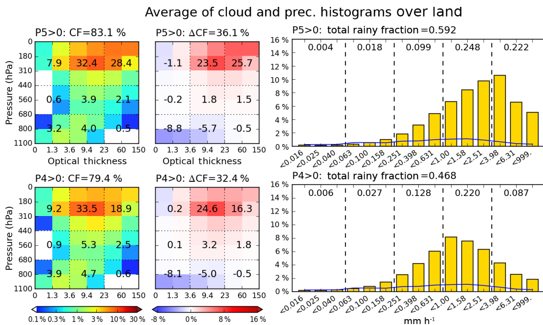
Figure 6. Same as Fig. 5, but over land.
