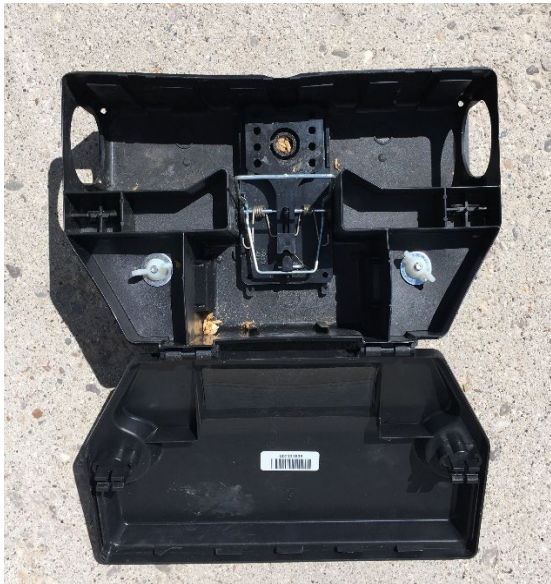
Figure 4. This Liphatech Aegis® bait station can hold a rat-sized snap trap.
