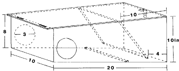
Figure 6. Wood bait station constructed of dimension lumber or exterior grade plywood or chipboard.
