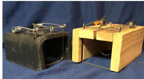
Figure 7. Box-style traps. (Left) The Victor® Black Box Gopher Trap and (Right) the DK-2 Gopher Getter Box Trap.
