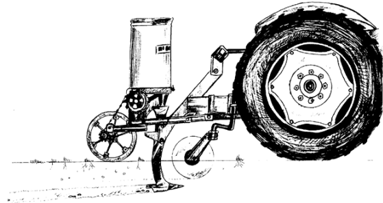
Figure 11. A pocket gopher burrow builder. The burrow builder meters out grain bait into an artificial burrow. Pocket gophers enter the artificial burrow where it intersects the natural burrow and find the bait.
