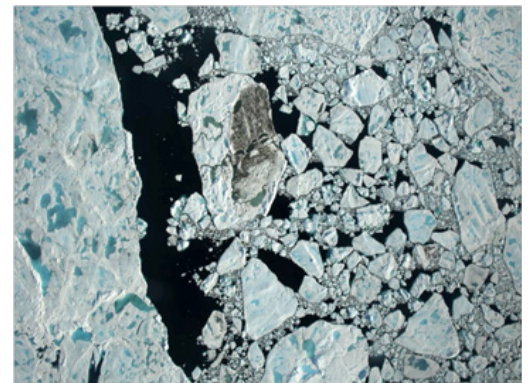
A DMS image of broken sea ice floes with blue melt ponds scattered throughout much of the surface. (NASA/Eric Fram)
