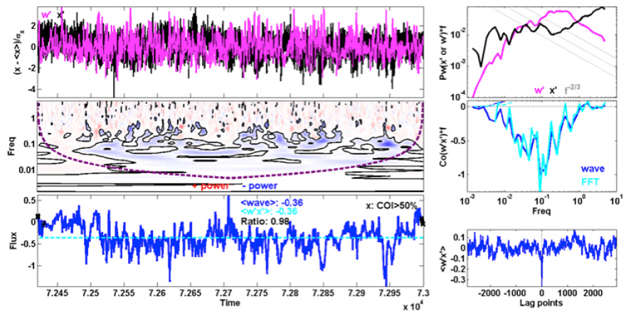
Example CO 2 flux data including wavelet analysis for one 10-min (25 km) leg at 500' largely over dense forest. Diagnostics confirm the frequency response and sensitivity of the instrumentation and quantify uncertainties. Much of the variability in the flux time series is repeatable and associated with conditions on the ground, which will be analyzed in more detail.
