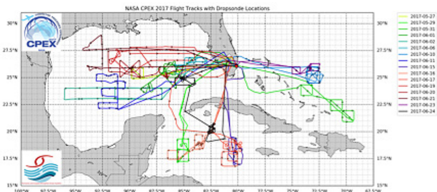
Flight tracks of CPEX science missions (colored by date) with dropsonde locations (dots).
