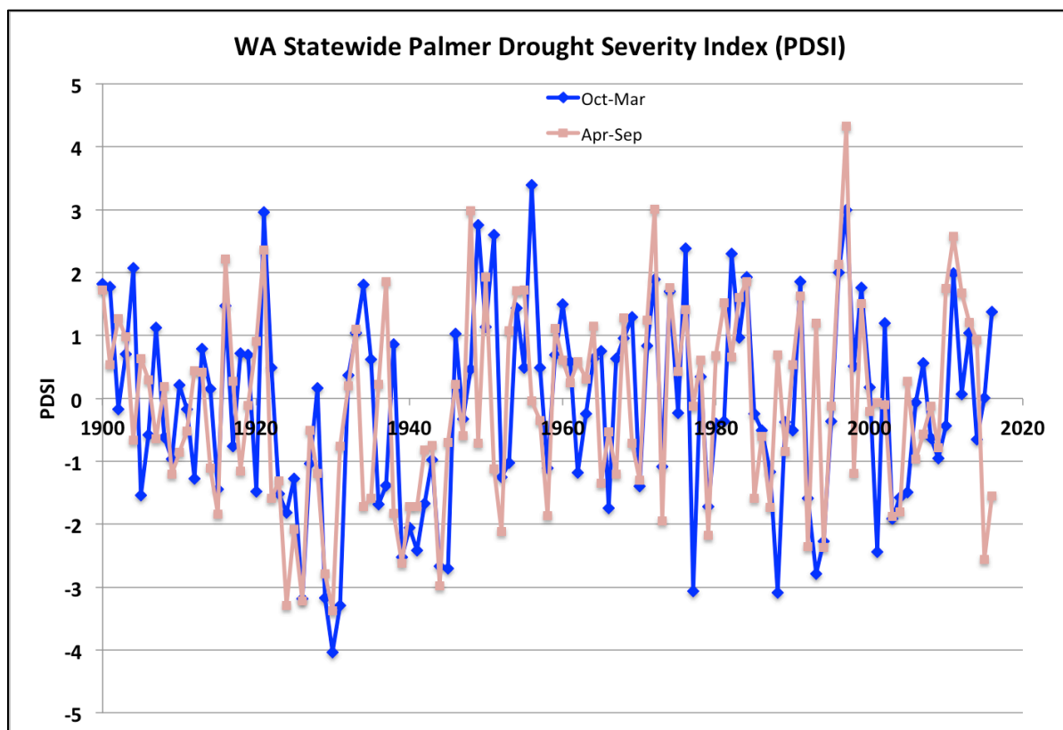
Figure 7. Time series of Palmer Drought Severity Index (PDSI) for Washington State 1900 to 2016 for October through March (blue line) and April through September (pink line).
