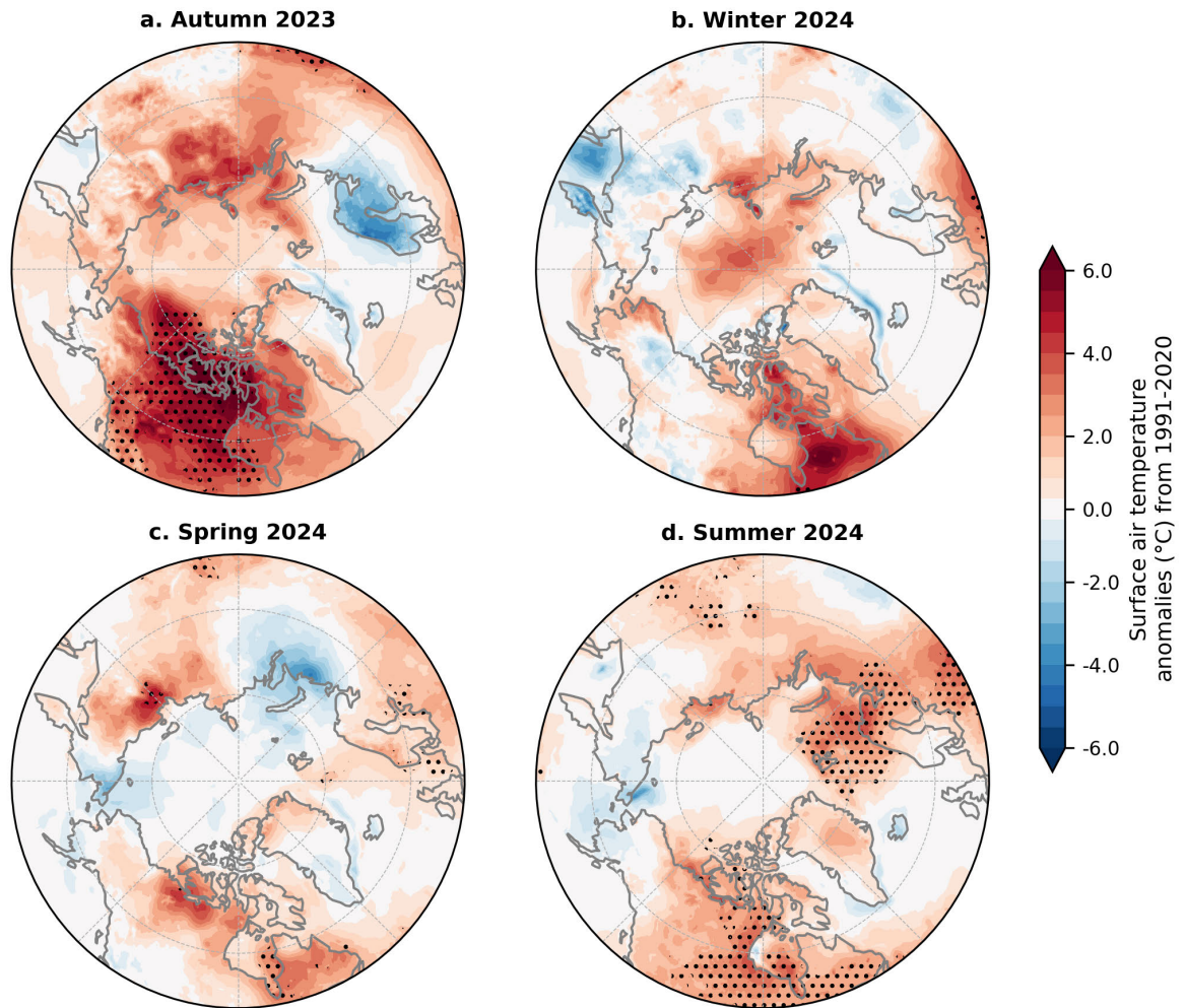
Fig. 2. Seasonal surface air temperature anomalies ( ^{\circ}\text{C} ) for (a) autumn 2023, (b) winter 2024, (c) spring 2024, and (d) summer 2024. Temperature anomalies are shown relative to their 1991-2020 means. Stippled areas indicate record high seasonal temperatures since 1950. Source: ERA5 reanalysis air temperature data are obtained from the Copernicus Climate Change Service.
