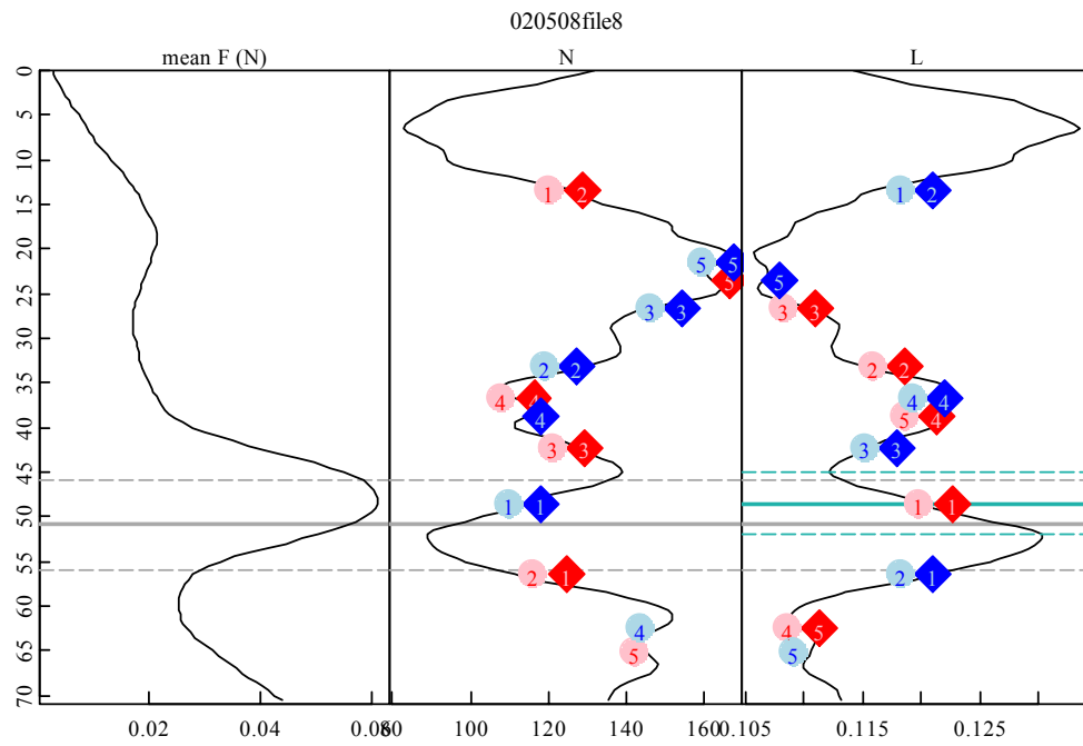
Figure 87: SMP Profile #7.
