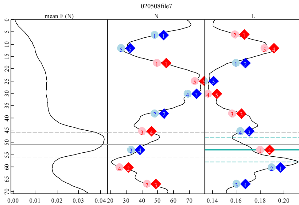
Figure 86: SMP Profile #6.
