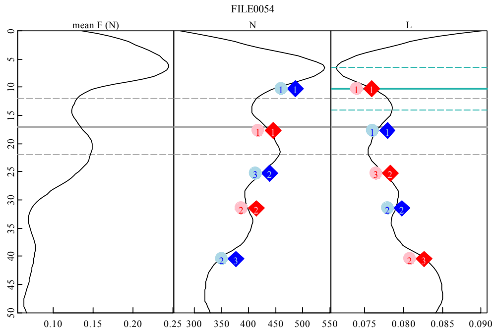
Figure 110: SMP Profile #30.
