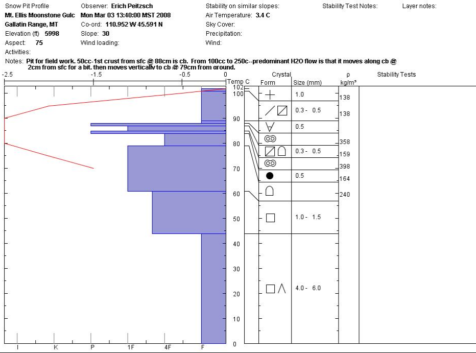
Figure 74: Pit profile #25.
