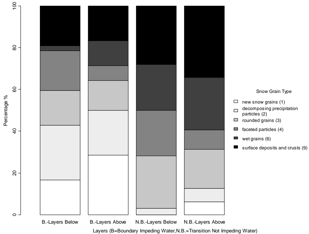
Figure 27: Relative proportions of crystal types comprising the layers above and below transitions that impeded water and transitions that did not impede water of all samples.
