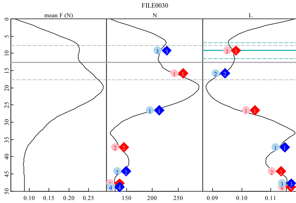
Figure 104: SMP Profile #24.
