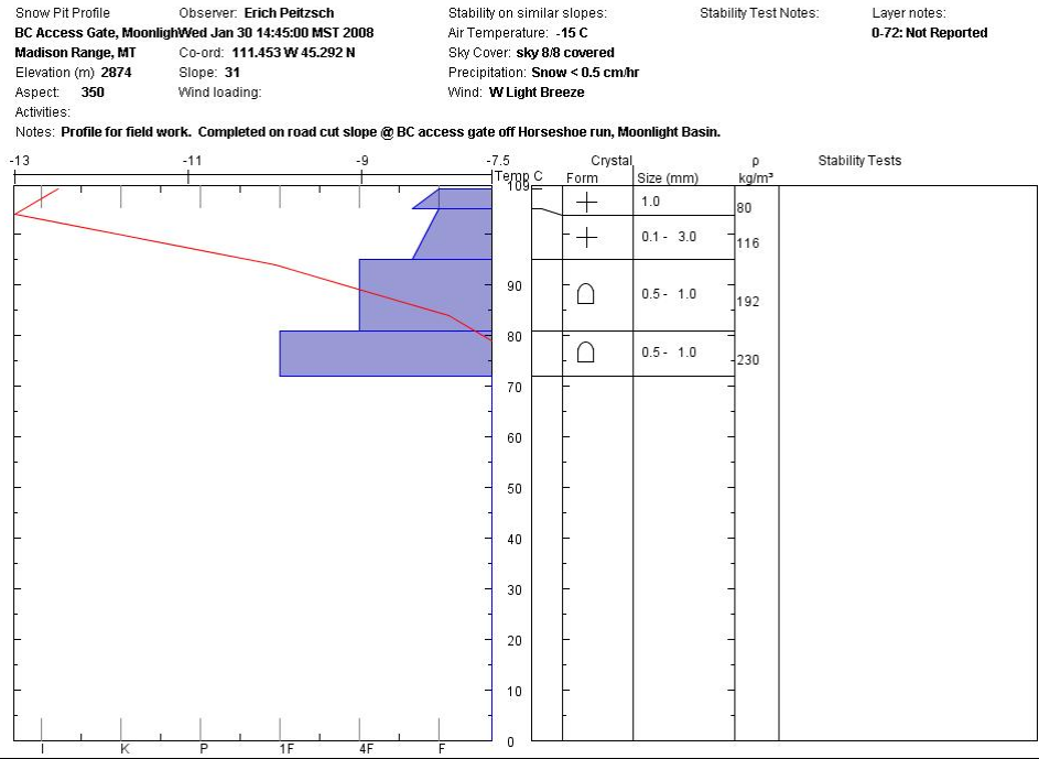
Figure 54: Pit profile #5
