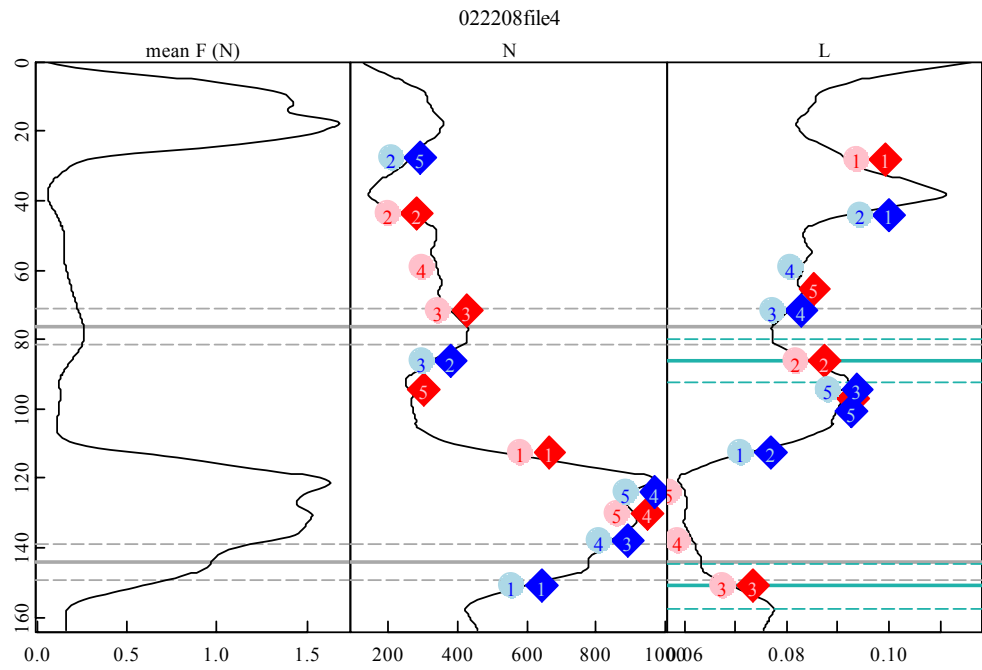
Figure 92: SMP Profile #12.
