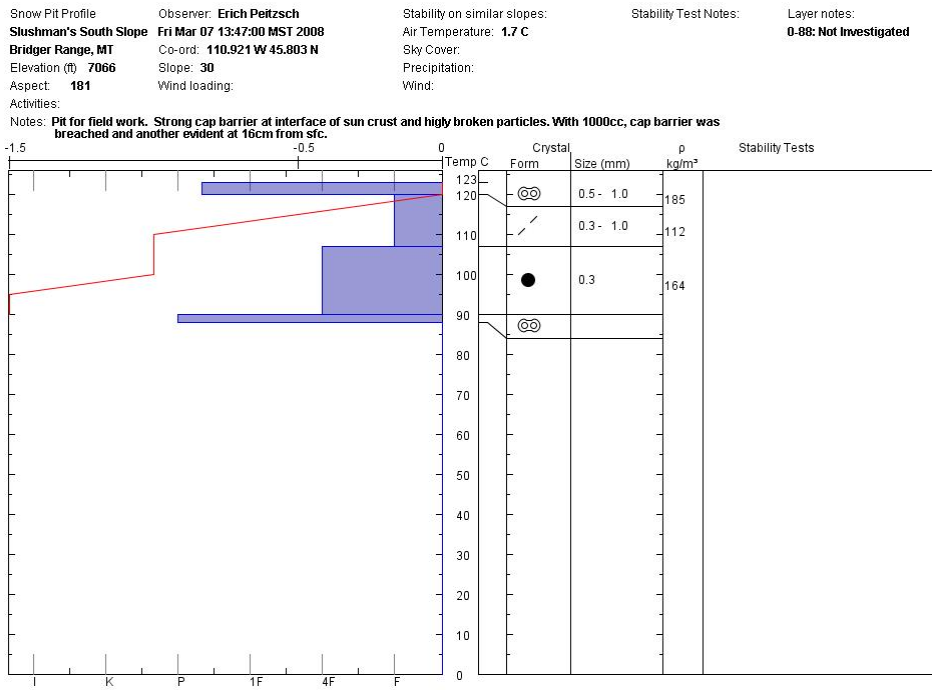
Figure 75: Pit profile #26.
