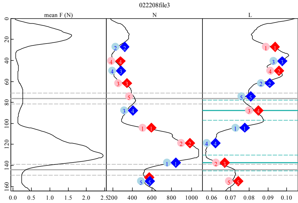
Figure 91: SMP Profile #11.
