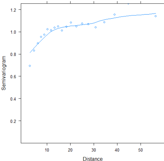
Figure 5: Semivariogram of the data from our study, which we fit with a spherical correlation model.
