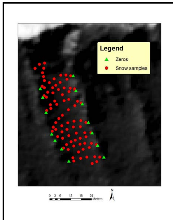
Figure 3: Example of sampling scheme showing snow observations and couloir boundary locations (denoted by the zero points).
