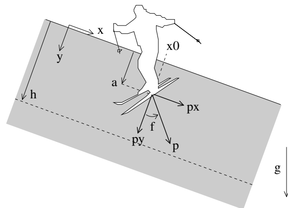
Figure 1. A skier with instant position x_0 sinks into a slab of thickness h by an amount a < h . Under plain strain conditions, he/she acts as a line load with slope-parallel component p_x and slope-normal component p_y . The load causes an additional compressive stress \sigma(x) and shear stress \tau(x) at an arbitrary point in the weak layer plane. The direction f of the applied load is arbitrary (not necessarily parallel to the acceleration of gravity g ).
