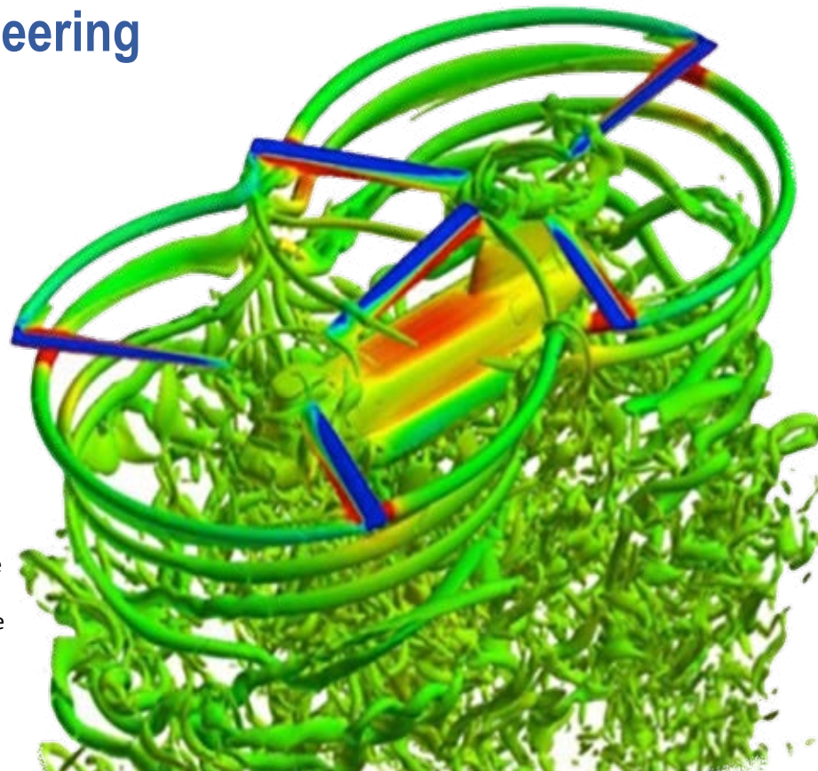
Figure 1: CH-77 Rotor Vortices in Helios
