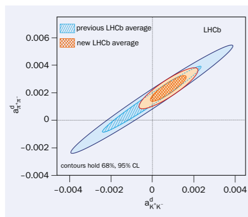
Fig. 1. Preliminary plot of the contours showing the measurement of the direct CP asymmetry for the decays D^0 \rightarrow \pi^+ \pi^- versus D^0 \rightarrow K^+ K^- . The new measurement of a_4(D^0 \rightarrow K^+ K^-) improves the precision significantly and leads to evidence that a_4(D^0 \rightarrow \pi^+ \pi^-) is different from zero. The inner (outer) ellipses show the 1 (2) \sigma contours.
