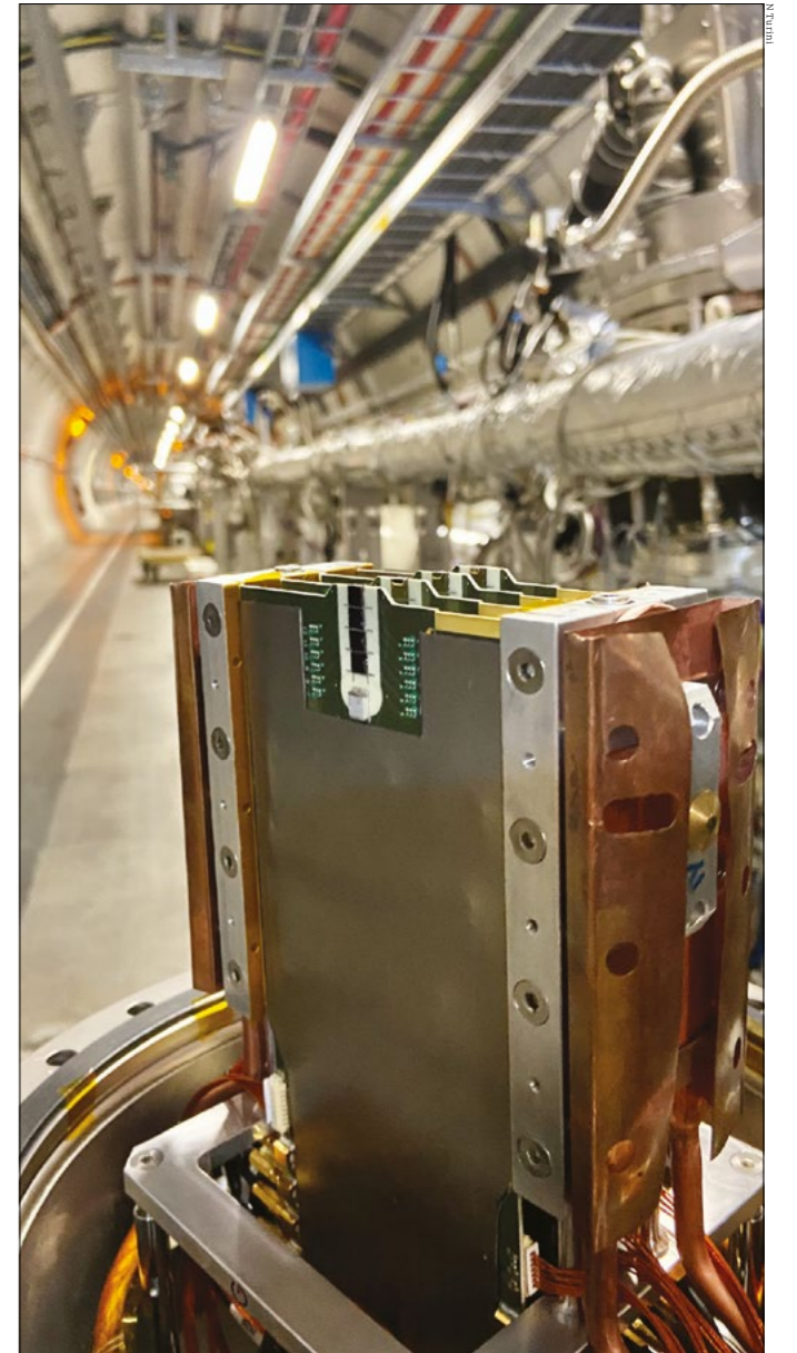
Timing detectors The new PPS timing detector just before installation inside a Roman Pot. The sensitive elements are the dark crystals seen on the top part of the detector, made from synthetic diamond, with a total active surface of 4.5 \times 18 \text{ mm}^2 per plane.
