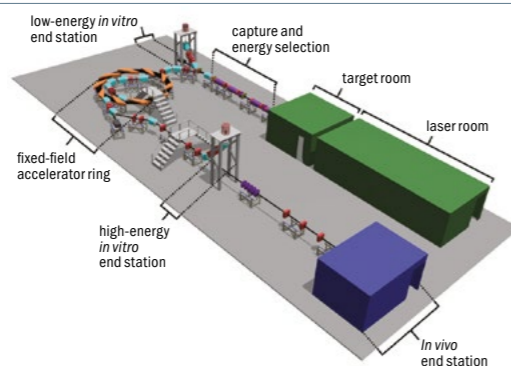
Ambitious Schematic showing the layout of the proposed Laser-hybrid Accelerator for Radiobiological Applications (LhARA).
