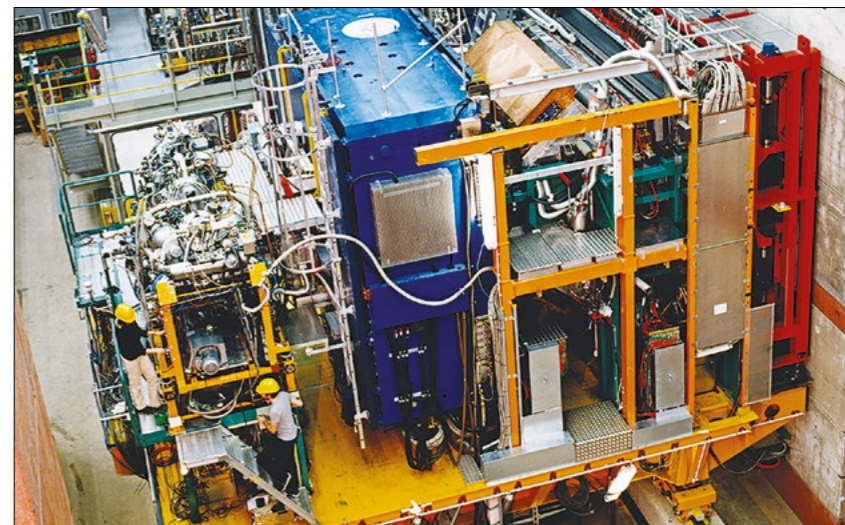
Spin messenger The former HERMES detector at DESY's HERA collider collected data from the scattering of longitudinally polarised electrons on various polarised and unpolarised gas targets.
