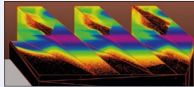
Synchrotron simulation Molflow simulation of the synchrotron-radiation power density on a “crotch absorber”, which protects downstream UHV vacuum chambers in a storage ring.
