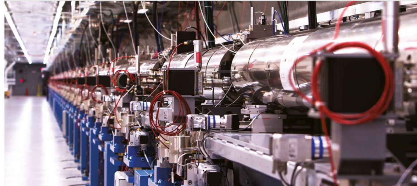
Intense The LCLS undulator hall, where high-energy electrons run a gauntlet of 32 undulators each containing 224 magnets whose alternating poles force the electrons to zigzag violently and radiate X-rays. (Credit: SLAC)
