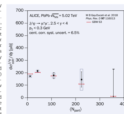
Fig. 1. J/\psi photoproduction cross section as a function of the mean number of nucleons participating in hadronic PbPb interactions, \langle N_{part} \rangle , at a centre-of-mass energy of 5.02 TeV. The results are compared with theory predictions from a UPC-like calculation accounting for the nuclear overlap.
