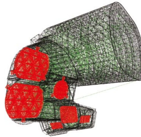
Molflow in space Above: a vacuum-chamber simulation performed for NASA's Mars 2020 mission. Left: designing a decontamination solution for NASA's SPHEREx mission, due for launch in 2024. (Credit: JPL Contamination Control Engineering)
