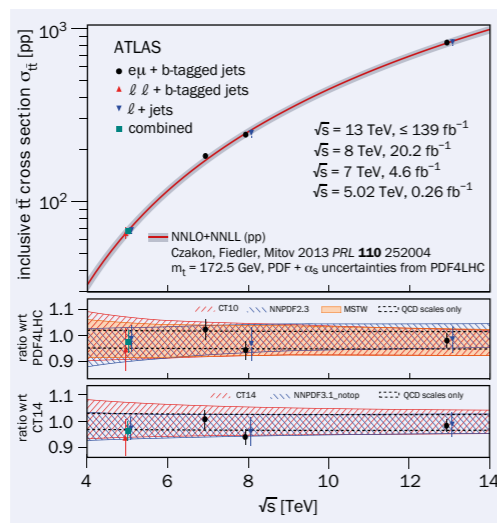
Fig. 1. ATLAS measurements of the t\bar{t} -production cross section as a function of centre-of-mass energy compared to the SM prediction, with measurements made at the same energy slightly offset for clarity. The middle and lower panels show the ratios of measurements and predictions from different parton-distribution functions.
