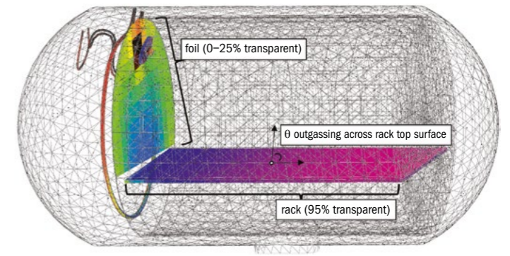
Molflow in space Above: a vacuum-chamber simulation performed for NASA's Mars 2020 mission. Left: designing a decontamination solution for NASA's SPHEREx mission, due for launch in 2024. (Credit: JPL Contamination Control Engineering)
