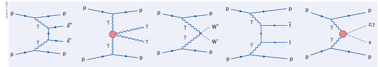
Photon fusion Diagrams showing different final states produced via photon-photon fusion probed by CMS.
