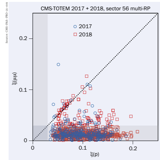
Tagging exclusive events When particles are produced exclusively, proton momentum loss \xi can be reconstructed from the central system or the intact proton. The dotted line illustrates the case of a perfect correlation, where exclusive events are expected.
