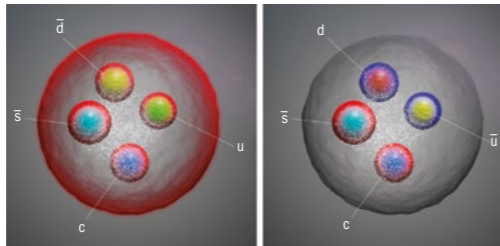
Brand new LHCb's latest tetraquarks, illustrated here as single units of tightly bound quarks, go by the names T_{cc}^+(2900) and T_{cc}^0(2900) in the new naming scheme.
