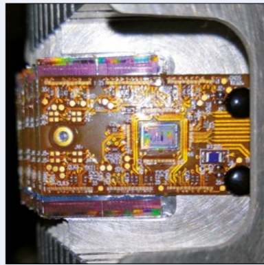
Tracking station Each detector plane contains a silicon pixel sensor coupled to four readout chips.
