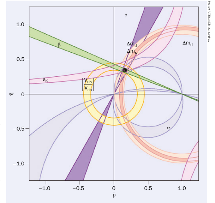
Testing quark mixing The unitarity triangle (defined by the angles \alpha, \beta and \gamma ), which exists in the complex \bar{p} - \bar{\eta} plane, represents a requirement that the Cabibbo-Kobayashi-Maskawa (CKM) matrix is unitary, meaning that the number of quarks is conserved in weak interactions and that there are only three generations of quarks. Its area is a measure of the amount of CP violation in the Standard Model. Checking the consistency of different measurements of the unitarity triangle is an important test of the Standard Model. At the apex of the triangle, closed contours at 68% and 95% probability are shown. Full lines correspond to 95% probability regions for each of the physical constraints, given, respectively, by the measurements of |V_{ub}|/|V_{cb}| from semileptonic b \rightarrow c and b \rightarrow u decays; the B_{d,s}^0 - \bar{B}_{d,s}^0 mixing amplitudes, \Delta m_d and \Delta m_s ; the K^0 - \bar{K}^0 CP violation parameter \epsilon_K ; the angle \alpha from B \rightarrow \pi\pi, B \rightarrow \rho\pi and B \rightarrow \rho\rho decays; \sin^2\beta from the measurement of the CP asymmetry in the J/\psi K^0 decays; and the angle \gamma from B \rightarrow D^{(*)}K^{(*)} decays.
