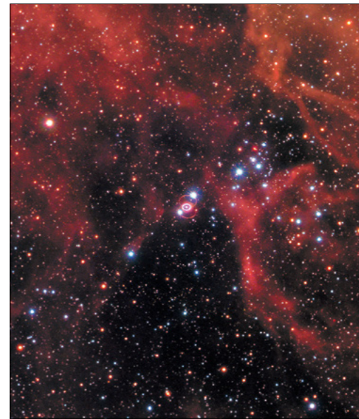
Treasure trove More than 35 years on, supernova 1987A (the double-ring structure at the centre of the image shows its remnant, as observed today) is still a topic of active discussion, including at Neutrino Platform Pheno Week.
