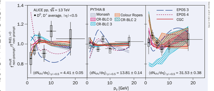
Fig. 1. The ratio between the fraction of non-prompt D^0 and D^+ mesons measured in three different multiplicity intervals and the multiplicity-integrated fraction in pp collisions at a centre-of-mass energy of 13 TeV. The PYTHIA 8 curves obtained with different tunes describe the data satisfactorily, except for the CR-BLC3 (cyan), which underestimates the ratio between non-prompt fractions at low p_T for the high-multiplicity class of events.
