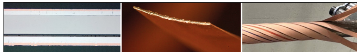
Bridging the gap Shown on the left is a longitudinal cross-section of 4 mm-wide REBCO tape, pictured from a different perspective in the middle panel, and on the right is a 10 mm-diameter REBCO cable for 3 kA currents at 60 K.
