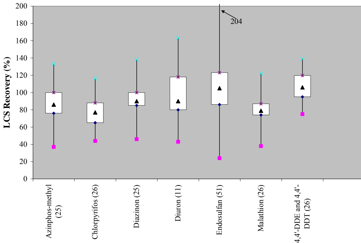
Figure C-2. LCS performance, 2004-2005.
