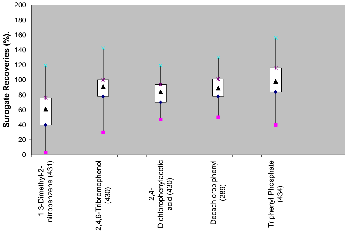
Figure C-1. Surrogate recovery.
