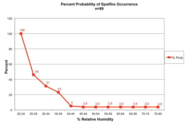
Figure 4. Probability of spotfire occurrence increases below 40 percent relative humidity.
