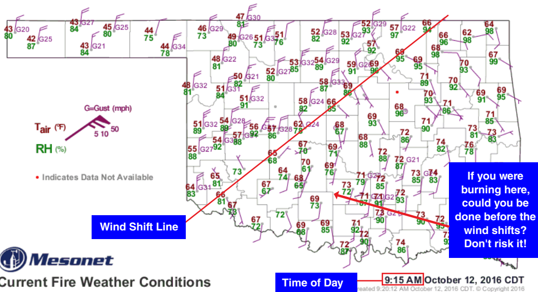
Figure 2. Do not burn within 12 hours of a predicted wind shift or frontal passage. In the example above, a strong cold front is crossing the state with an abrupt shift in wind directions.
