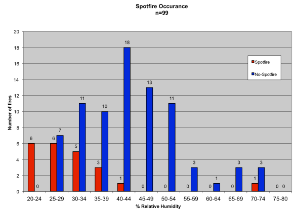
Figure 3. Spotfires can occur at any time, but the majority happen when relative humidity is below 40 percent.
