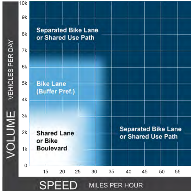
Preferred Bikeway Type for Urban, Urban Core, Suburban and Rural Town Contexts (2019). Source: FHWA Bikeway Selection Guide
