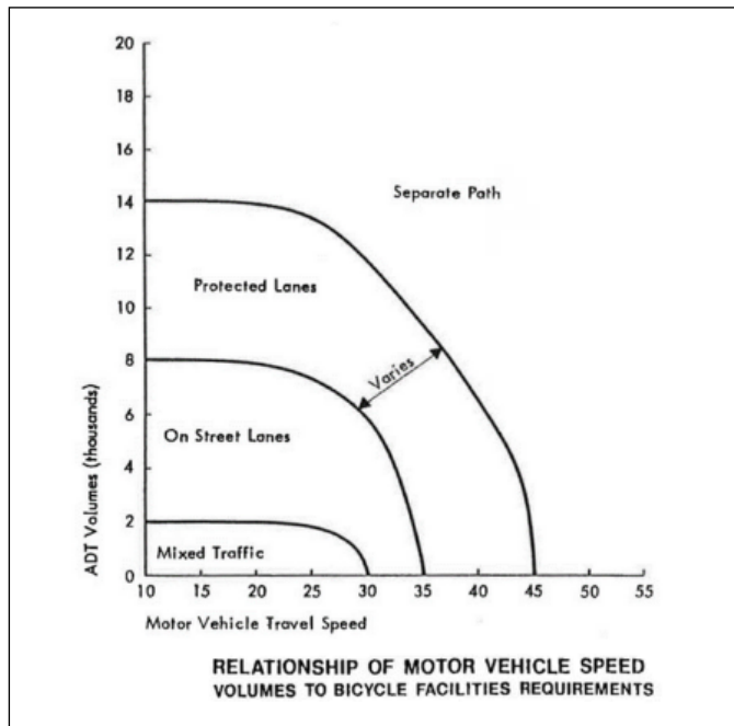
Bikeway selection graph for City of Davis, CA (1972). Source: FHWA Literature Review – Resource Guide for Separating Bicyclists from Traffic
