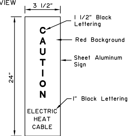
CAUTION SIGN
