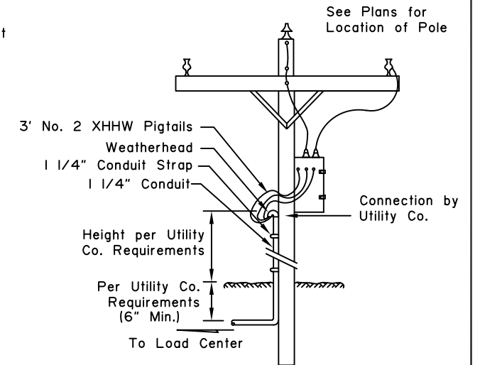
UNDERGROUND SERVICE POLE RISER DETAIL
