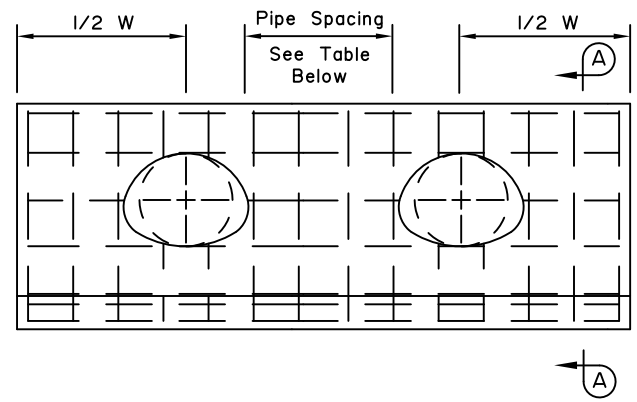
MULTIPLE INSTALLATION
