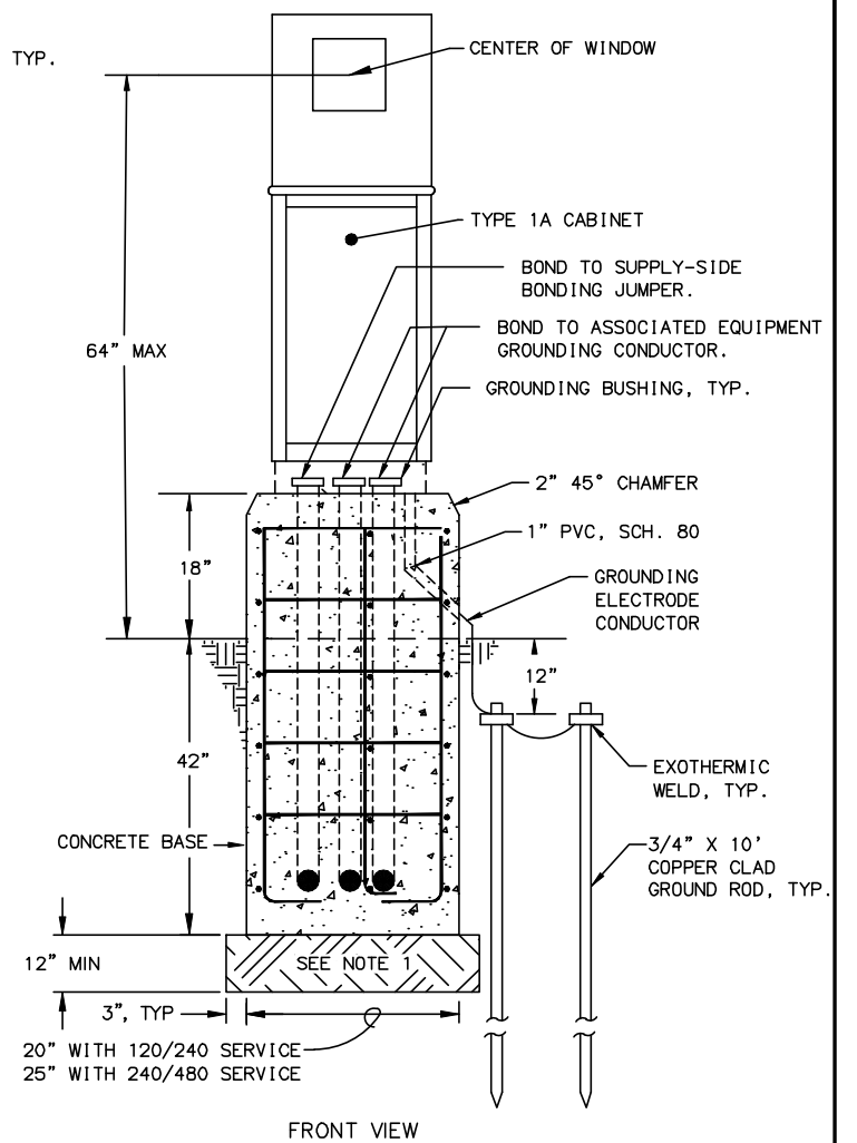
TYPE 1A LOAD CENTER BASE DETAILS
