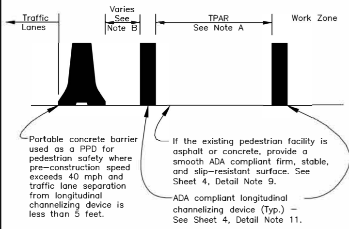
PEDESTRIAN DIVERSION TYPICAL SECTION
