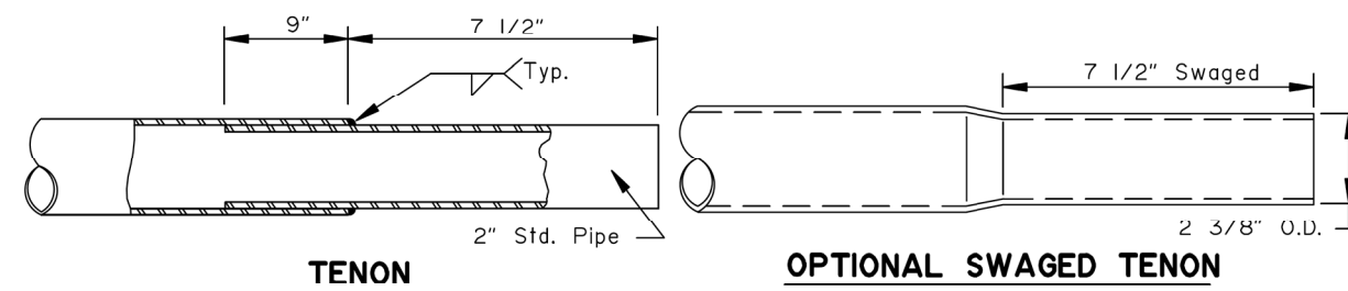
END OF MAST ARM DETAIL
