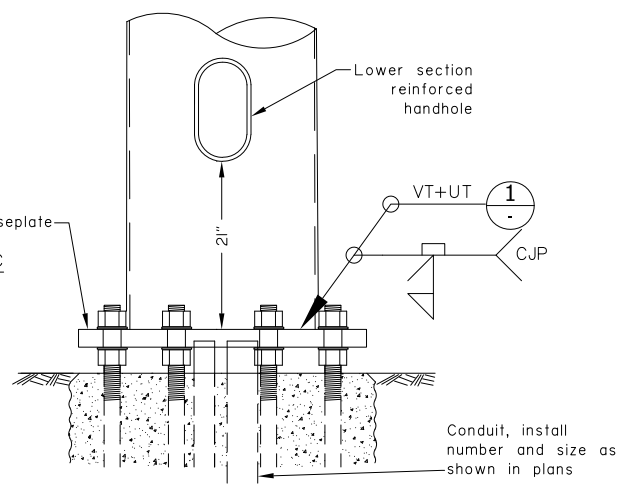
FRONT VIEW (Skirt omitted for clarity)
