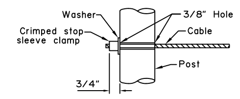
ALTERNATIVE DEAD END ANCHORAGE
