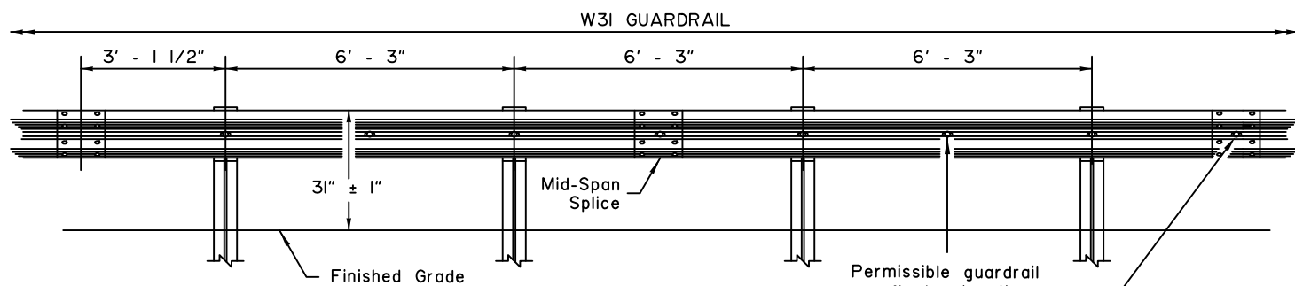
TYPICAL ELEVATION
