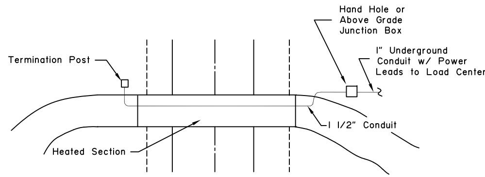
PLAN
