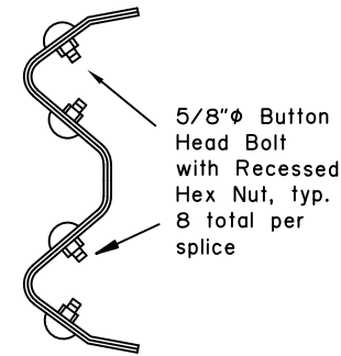
SPLICE CROSS-SECTION
