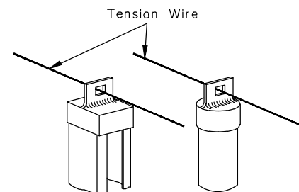
LINE POST TOPS
