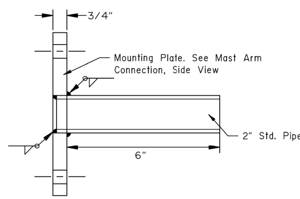
TENON MOUNT DETAIL
