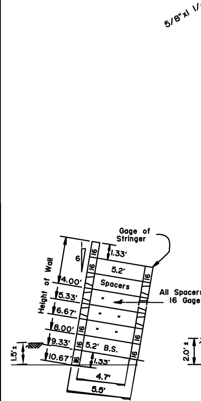
BIN WALL ASSEMBLY DETAILS
