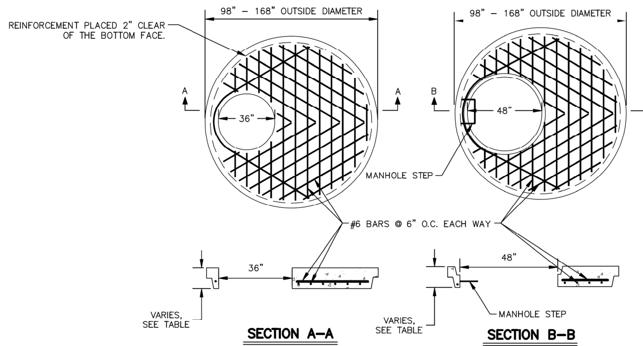
PRECAST CONCRETE REDUCING SLAB (84"-144" TO 36") N.T.S.
