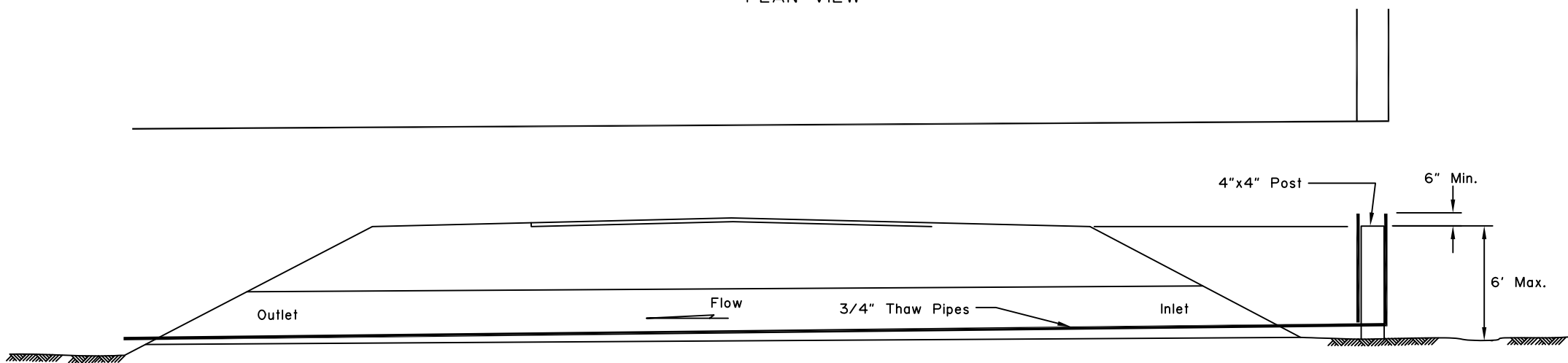
CROSS-SECTION
