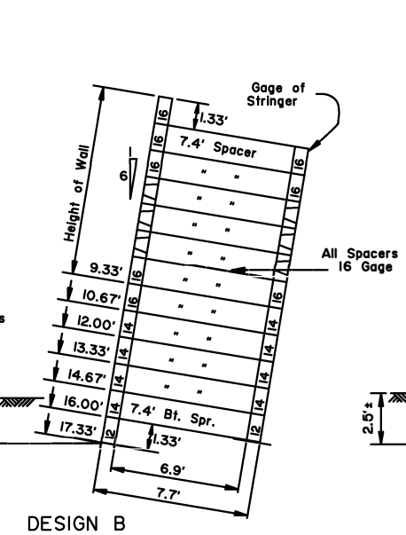
BIN WALL ASSEMBLY DETAILS
