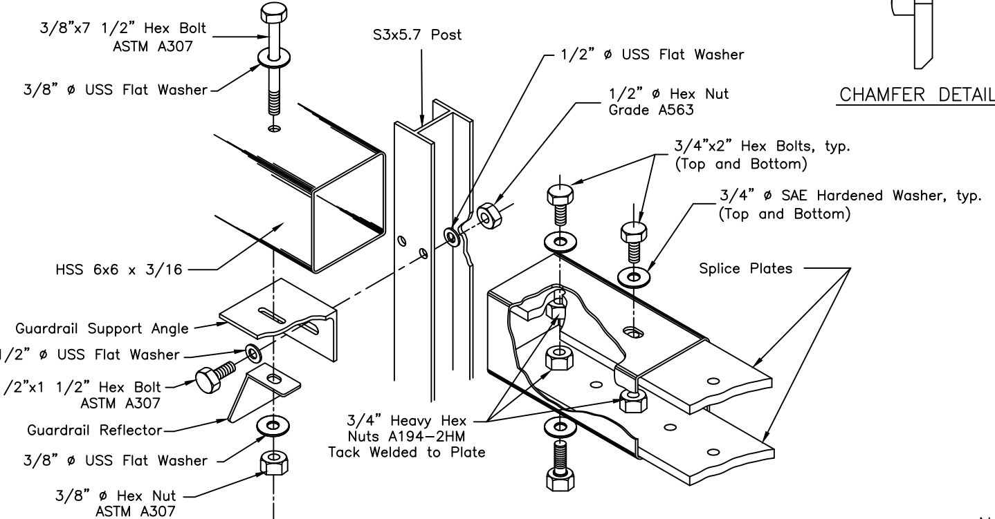
ASSEMBLY DETAIL
