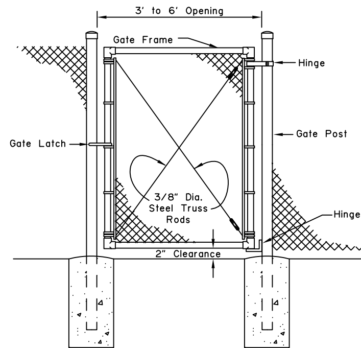
PEDESTRIAN GATE
