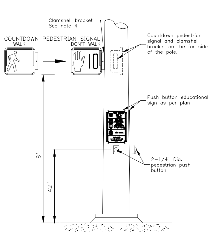
PEDESTRIAN HARDWARE
