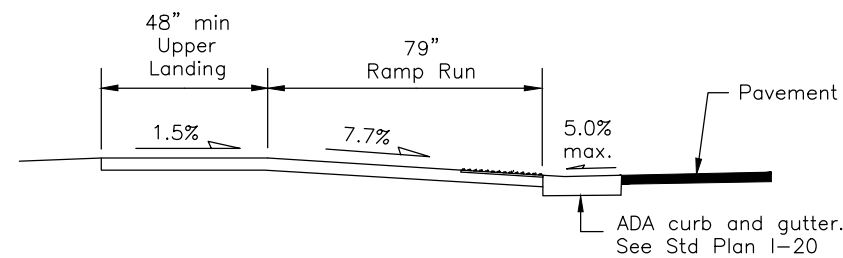
SECTION B-B
