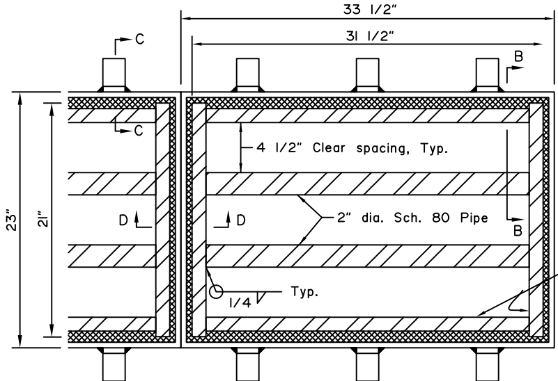
STEEL FRAME AND GRATE CONFIGURATION
