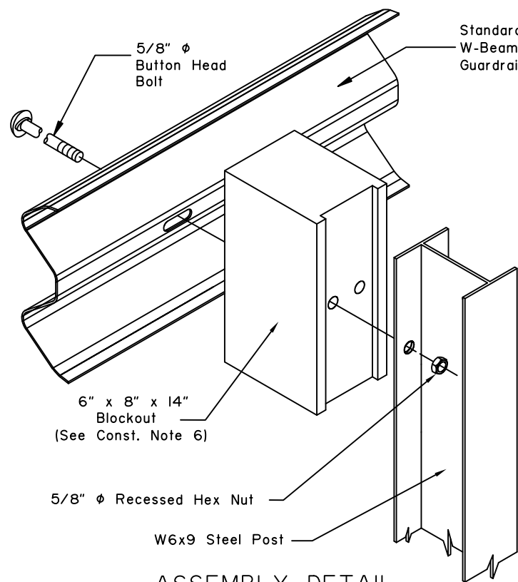
ASSEMBLY DETAIL
