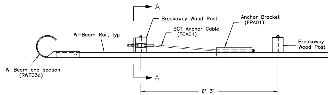
PLAN VIEW
