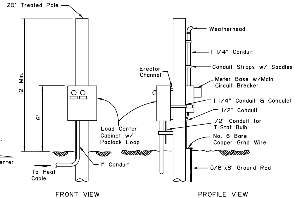
OVERHEAD SERVICE DETAIL
