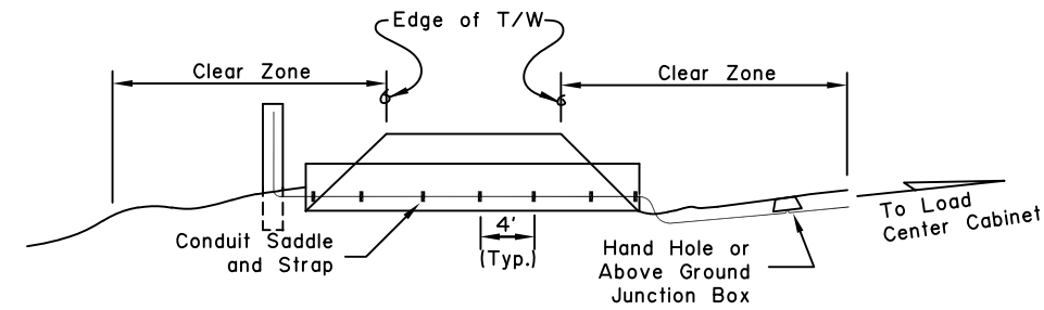
PROFILE
