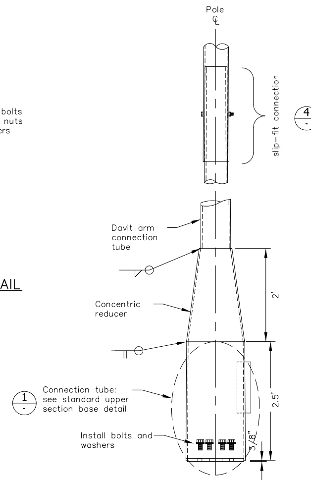
DAVIT UPPER SECTION BASE DETAIL NTS
