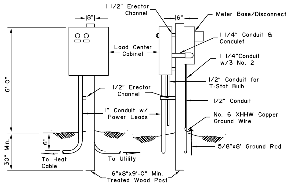
FRONT VIEW
