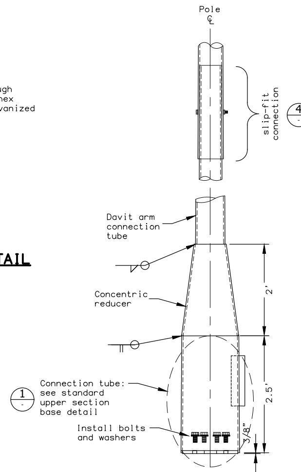
DAVIT UPPER SECTION BASE DETAIL
