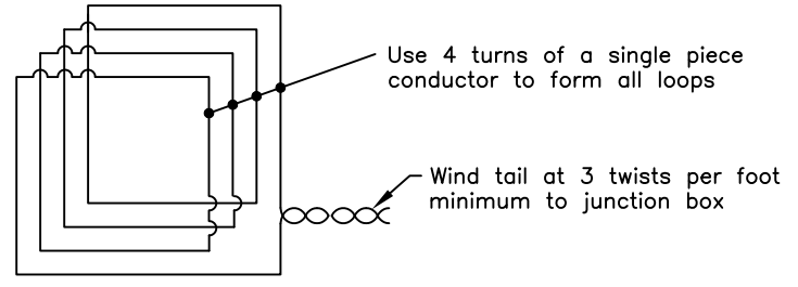
LOOP WIRING DETAIL
