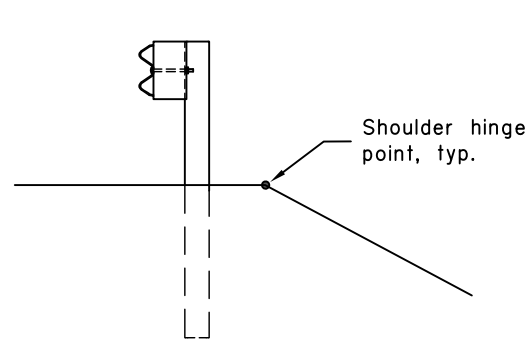
SECTION A-A Typical Section of Guardrail Installation at shoulder
