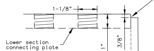
4b POST TOP LOWER SECTION CONNECTING PLATE
