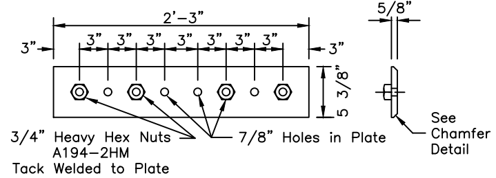
SPLICE PLATE
