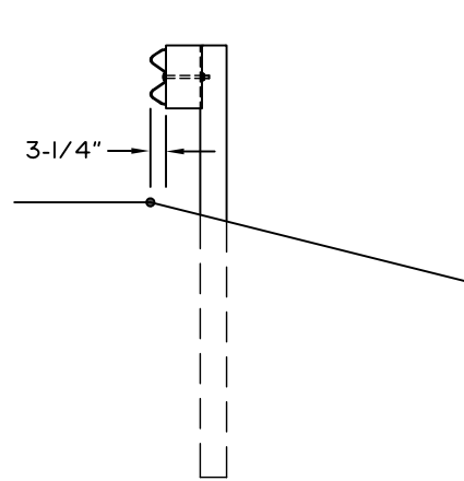
SECTION B-B Typical Section at Post I. Face of Guardrail flush with shoulder hinge point.
