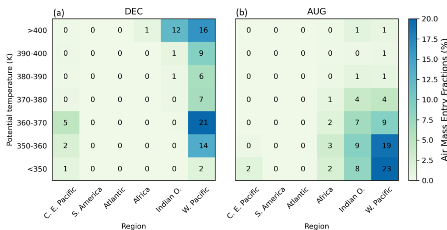
Figure 8. The air mass entry fractions (AEF) in (a) December 2018 and (b) August 2022. Calculations are based on the 10-d trajectory analysis (compare 6).
