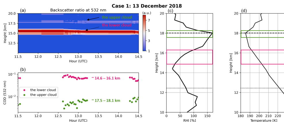
Figure 2. Lidar and radiosonde observations a typical case of cirrus cloud measurements on 13 December 2018. (a) The backscatter ratio (BSR) at 532 nm as a function of time and altitude. (b) The cloud optical depth (COD) at 532 nm of the upper and lower cloud layers as a function of time corresponds to Fig. 3a. (c) The relative humidity with respect to ice (RH i ) profiles as a function of height. (d) the temperature profiles as a function of height. The temperature and RH i profiles are obtained from the radiosondes launched at the Palau weather station (see Section 2). The horizontal lines indicate the altitude range of the TTL between the CPT height (dashed line, upper boundary of the TTL) and the height of LMS (level of minimum stability, dotted line, lower boundary of the TTL) calculated by the temperature profiles each day. Two cloud layers are marked by the box in the profile plot (c) and (d), with the same color code as in (b): the lower cloud marked as magenta and the upper cloud marked as green.
