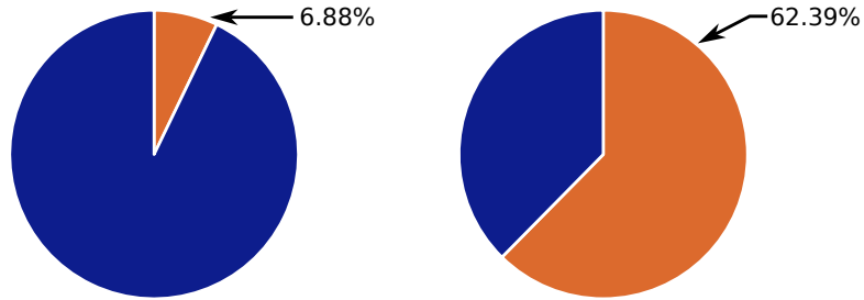
Fig. 1: Relative cost of SHAKE in key pair generation (left) and signature verification (right). This uses the BUFF variant of the verification.
