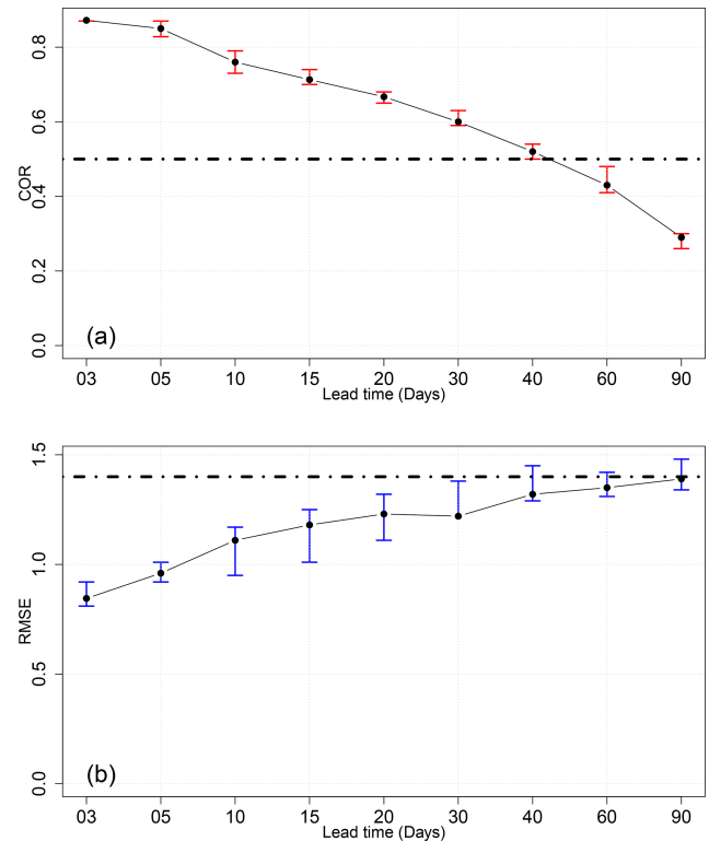
Figure 8. The COR (a) and RMSE (b) for the different lead times of forecasts from 3 to 90 d over the period from 1979 to 2020. Confidence intervals are obtained with a bootstrap with 1000 samples.
