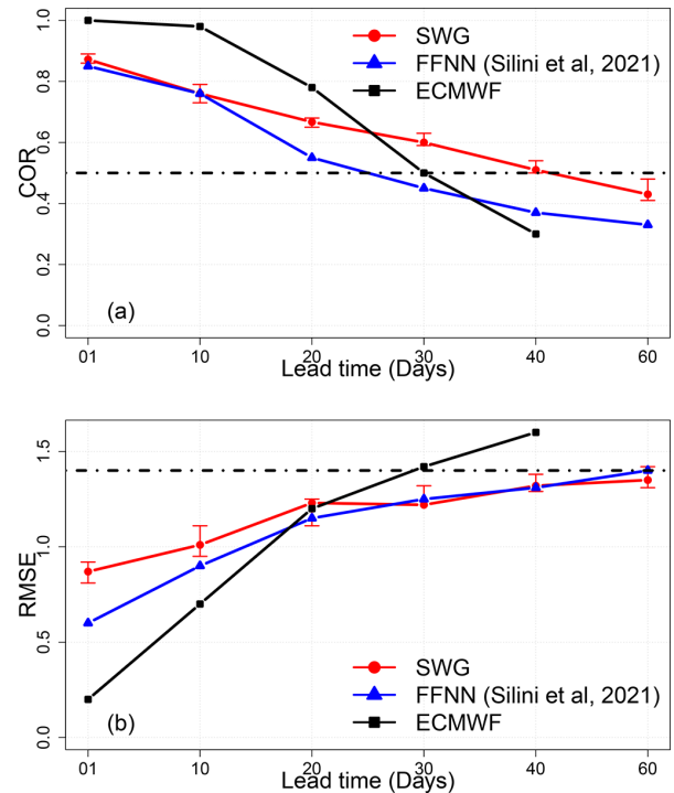
Figure 12. Comparison of the values of COR (a) and RMSE (b) between the SWG forecast and forecasts of Silini et al. (2021) (blue lines) and the ECMWF (black lines). Confidence intervals for SWG (red lines) were obtained with a bootstrap procedure over the simulations (1000 samples).
