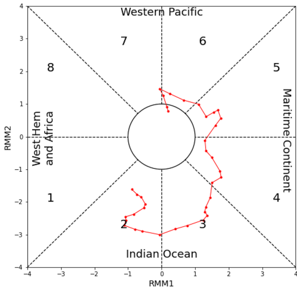
Figure 1. Wheeler–Hendon phase diagram of the MJO event for the period between 3 March and 9 April 1986, for observations. The diagram shows the eight areas of activity of MJO starting from the Indian Ocean.
