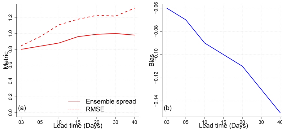
Figure 9. (a) Comparison between the ensemble spread and the RMSE. We note that the difference is small for short lead times ( \leq 15 d). “Metric” on the vertical axis refers to ensemble spread and RMSE. (b) The bias between the simulations and the observations for the lead times going from 3 to 40 d.
