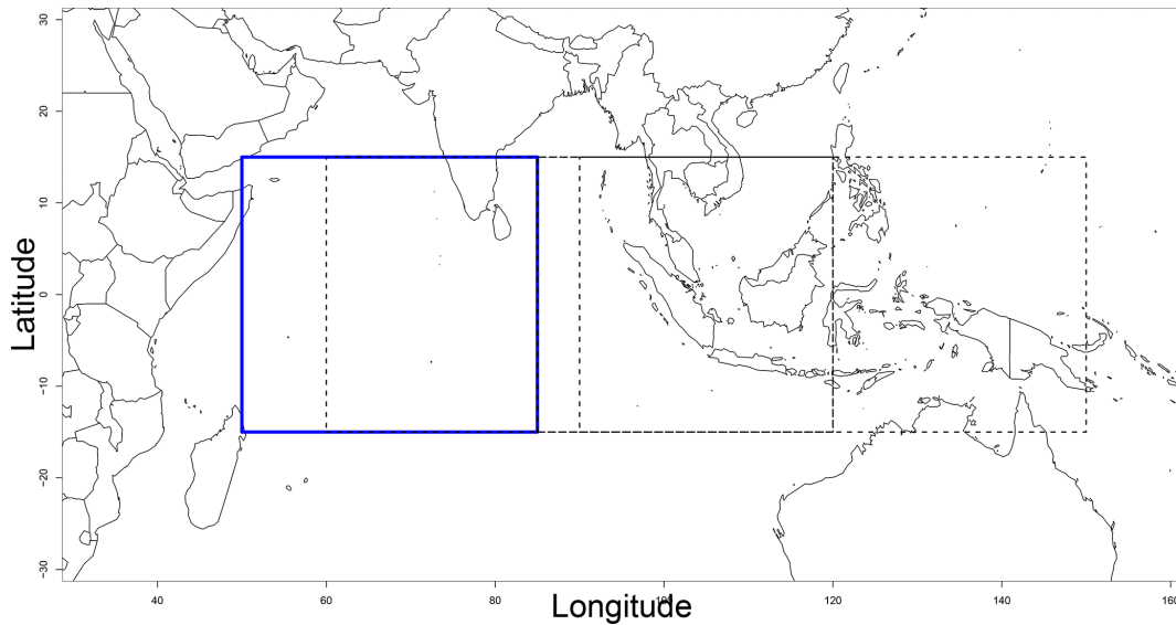
Figure B1. Domains of computation of analogs. We computed analogs over the Indian Ocean with coordinates 15° S–15° N, 50–85° E (blue rectangle); the Indian and Pacific oceans with coordinates 15° S–15° N, 85–120° E; and the Indian Ocean–Maritime Continent region with coordinates 15° S–15° N, 90–150° E.
