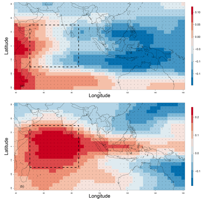
Figure 2. The optimal domain of computation of analogs. We computed analogs over the Indian Ocean, in the geographic areas indicated by the dashed black rectangle with coordinates 15^\circ\text{S} – 15^\circ\text{N} , 50 – 85^\circ\text{E} . The figure shows the temporal correlation between Z500 , RMM1 (a), and RMM2 (b) for the whole studied period from 1979 to 2020. The correlation is weak, but it is still significant, with p values \leq 0.05 that we indicate with black dots over each grid of the considered domain (including the optimal region used to compute analogs).
