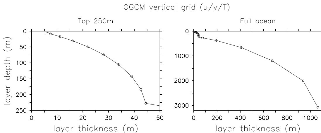
Figure F.2: Vertical grid of the ocean general circulation model. Gridpoints of temperature and horizontal velocity lie at the depths indicated by the circles; layer thicknesses are indicated on the horizontal axis. The vertical velocity grid is staggered in the vertical with respect to the grid shown.
