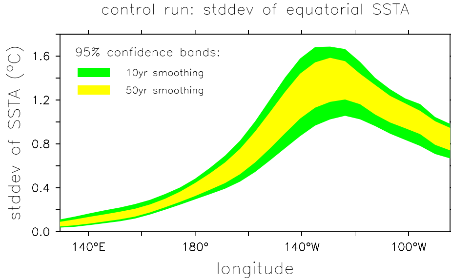
Figure 7.21: Confidence bands for the running standard deviation of SST anomalies along the equator ( 2^{\circ}\text{S} – 2^{\circ}\text{N} ) in the control run of the stochastic intermediate model. The standard deviation is computed by high-pass filtering the SSTA to eliminate periods longer than 8 years, squaring the result, low-pass filtering, and then taking the square root. The shaded bands are 95% confidence intervals for the standard deviation for a low-pass filter that eliminates periods shorter than 10 years (green) or 50 years (yellow).
