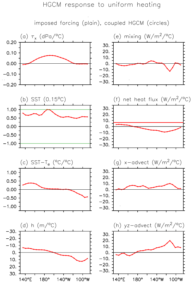
Figure 5.18: Response of the equatorial (2°S–2°N) climatology to an imposed uniform 1 W m -2 heating perturbation (plain line in panel f), as simulated by a hybrid coupled GCM. Fields are scaled by the peak SST change indicated in panel (b). Panels show the scaled change in (a) zonal stress, (b) SST, (c) temperature difference across the top 50 m, (d) depth of the 20°C isotherm (ordinate reversed); and the mixed layer heating due to (e) eddy fluxes, (f) surface fluxes, (g) zonal advection, and (h) meridional plus vertical advection.
