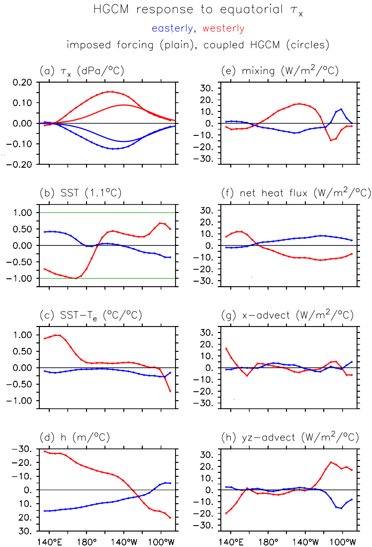
Figure 5.16: Response of the equatorial ( 2^\circ\text{S} – 2^\circ\text{N} ) climatology to an imposed equatorial zonal stress perturbation, as simulated by a hybrid coupled GCM. The imposed perturbation (plain lines in panel a) has a peak amplitude of 0.1 dPa on the equator at 140^\circ\text{W} and a bivariate Gaussian shape with e-folding halfwidths of 40^\circ longitude and 15^\circ latitude. Red (blue) lines correspond to a westerly (easterly) stress perturbations. Fields are scaled by the peak SST change indicated in panel (b). Panels show the scaled change in (a) zonal stress, (b) SST, (c) temperature difference across the top 50 m, (d) depth of the 20^\circ\text{C} isotherm (ordinate reversed); and the mixed layer heating due to (e) eddy fluxes, (f) surface fluxes, (g) zonal advection, and (h) meridional plus vertical advection.
