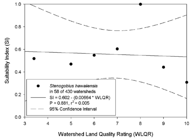
Figure 32. Suitability Indices for Watershed Land Quality Rating for Awaous guamensis , Lentipes concolor , Sicyopterus stimpsoni , and Stenogobius hawaiiensis .
