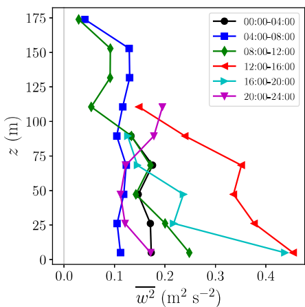
(f) Variance of vertical wind velocity
