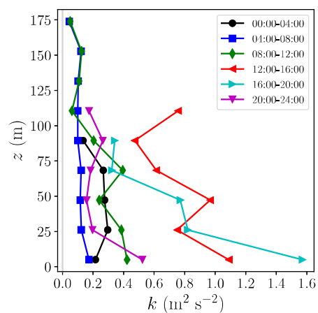
(a) Turbulence kinetic energy
