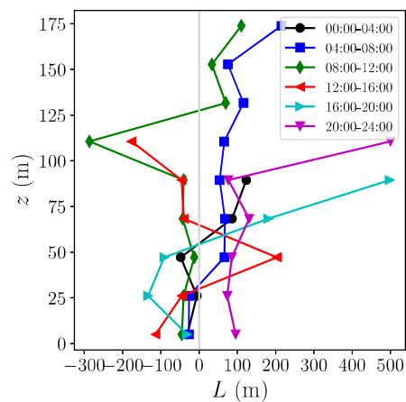
(c) Obukhov length
