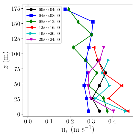
(b) Friction velocity
