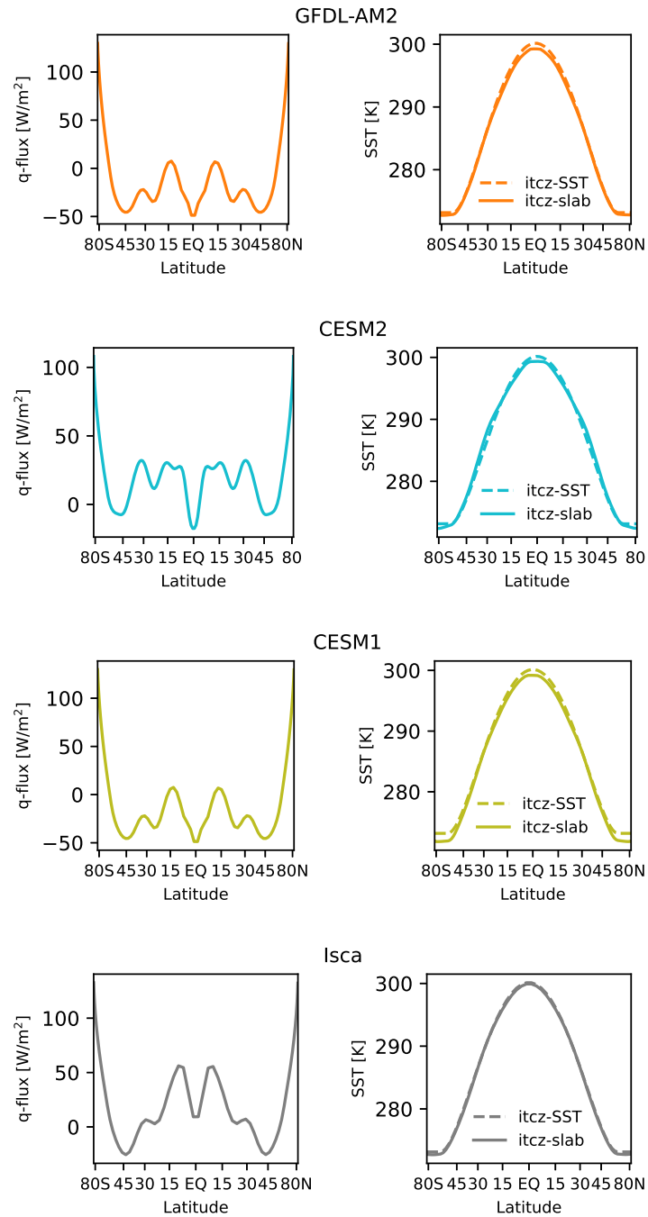
Figure S1. (left) Q -fluxes ( F in Eq. 2) derived from the itcz-SST prescribed SST experiment and applied to the itcz-slab control experiment for each model. (right) CONTROL prescribed SSTs and SSTs from the slab ocean control experiment, itcz-slab.
