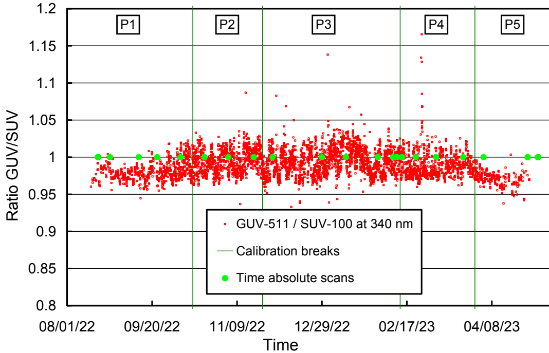
Figure 4. Ratio of GUV-511 (340 nm channel) and SUV-100 measurements. The times when “absolute” calibration scans of the SUV-100 were performed are indicated by green symbols.
