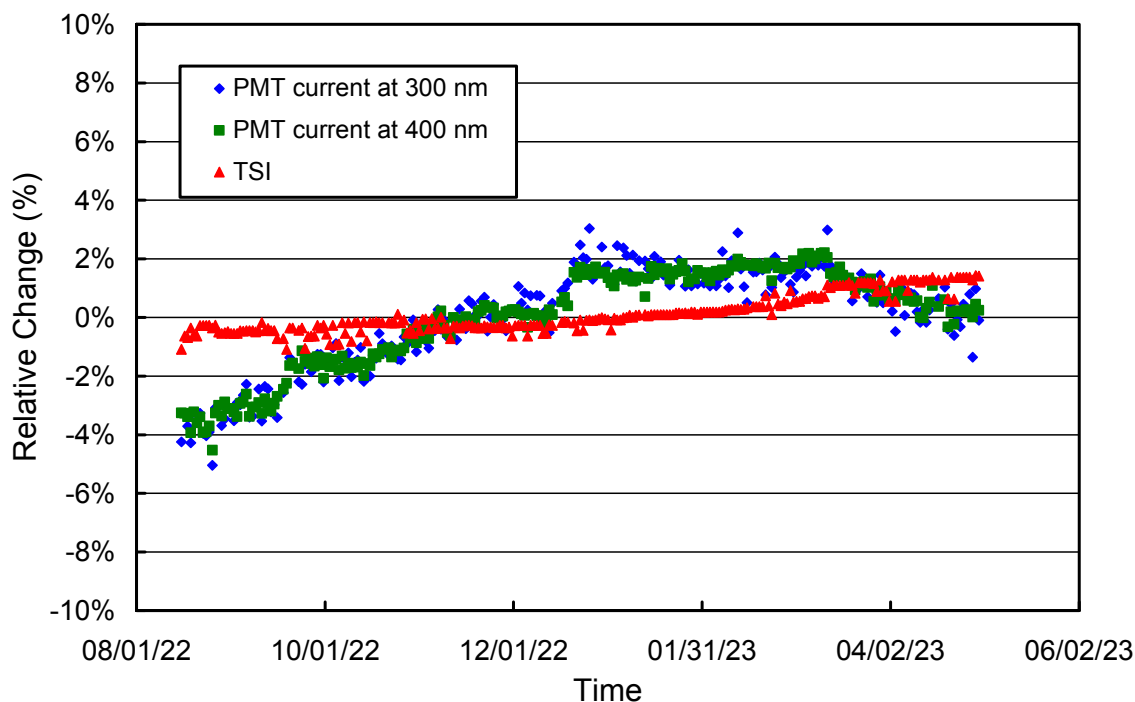
Figure 2. Measurements of the SUV-100’s TSI sensor and PMT currents at 300 and 400 nm. Data are shown as relative change and normalized to the average of the entire period.
