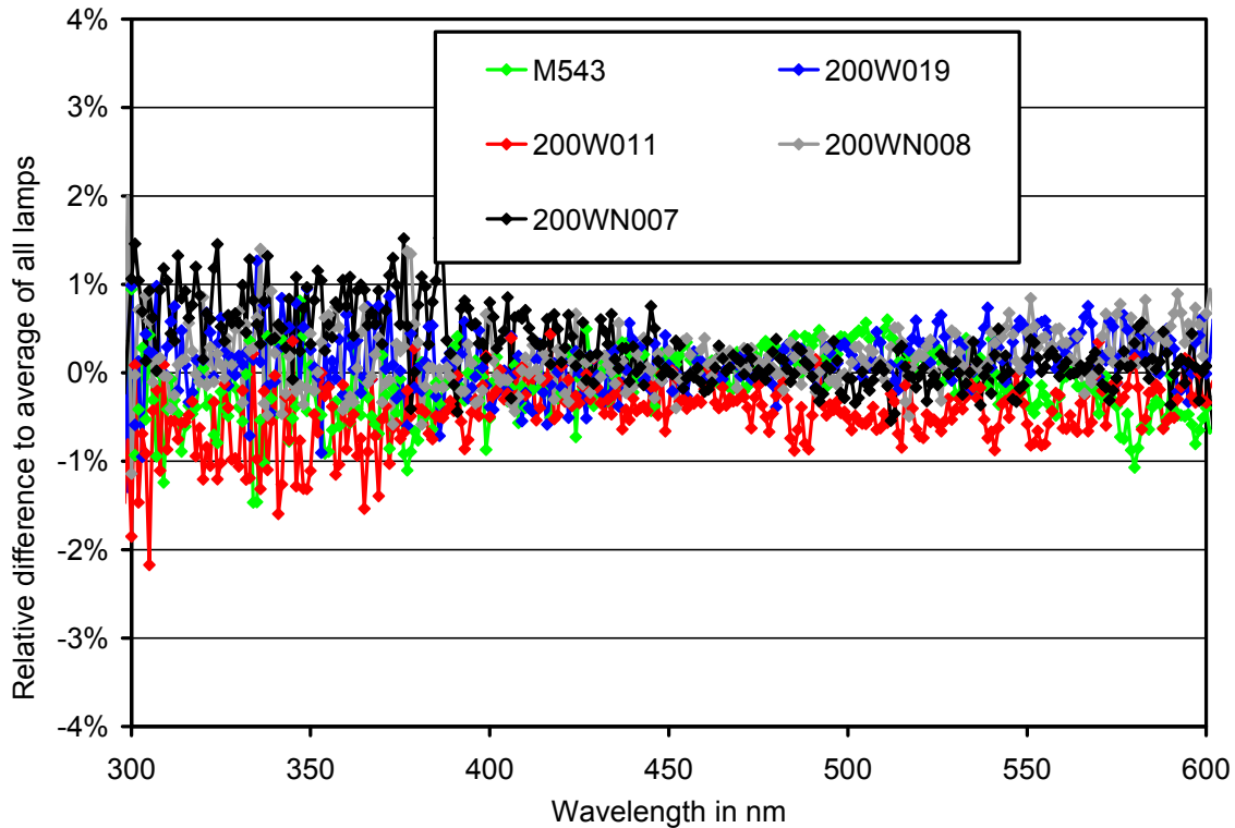
Figure 1. Comparison of all McMurdo working and long-term standards using absolute scans performed on 5/5/2023.
