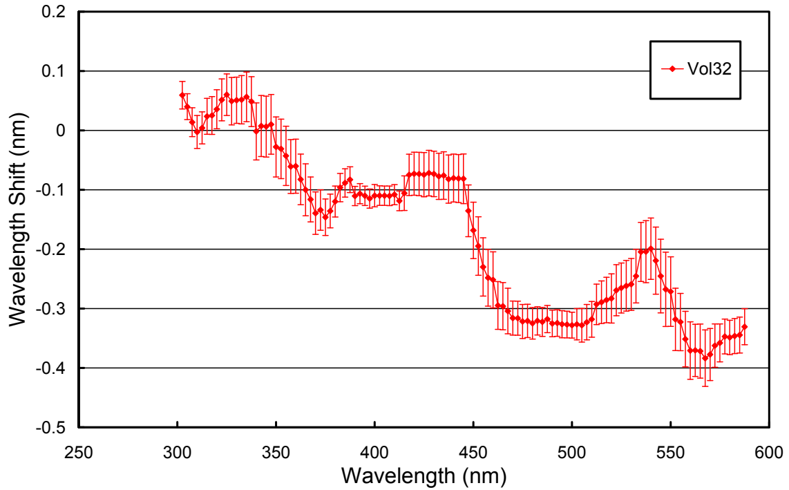
Figure 5. Monochromator non-linearity correction function for the Volume 32 period. Error bars indicate the 1\sigma -variation.
