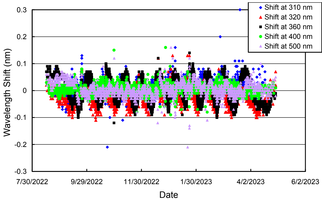
Figure 6. Check of the wavelength accuracy of Version 0 data at five wavelengths by means of Fraunhofer-line correlation. The plot is based on measurements that are one hour apart.
