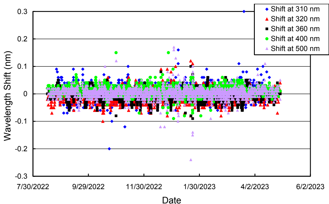
Figure 7. Check of the wavelength accuracy of Version 2 data at five wavelengths by means of Fraunhofer-line correlation.
