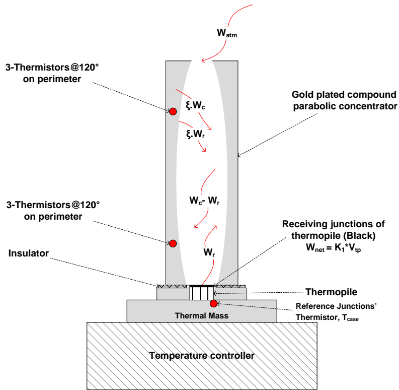
Absolute Cavity Pyradiometer (ACP)
