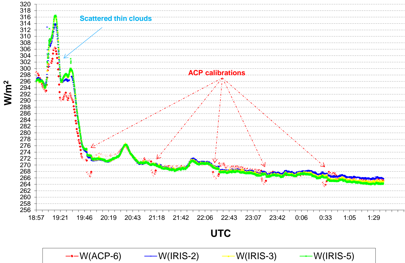
Night-Time IR irradiance measured at PMOD by ACP & IRIS on October 2&3, 2013 (~15 mm H 2 O vapor column)
