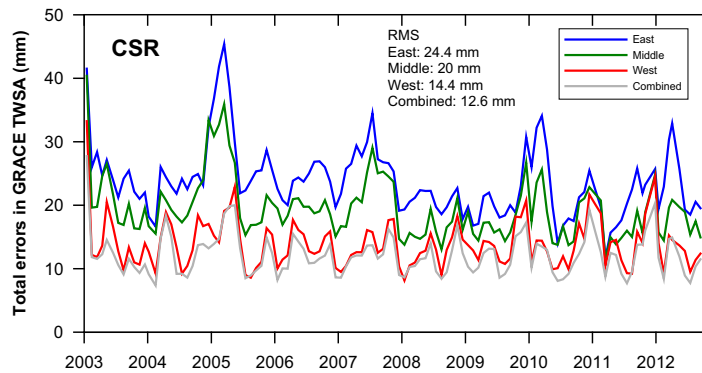
Figure 15. Time series of total error in GRACE-derived TWSA for the east, middle, west, and combined regions.
