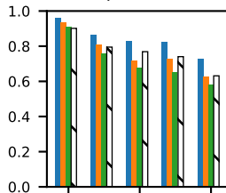
Alpha-NSE
