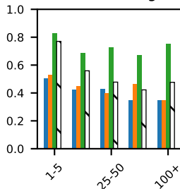
Peak-Timing
