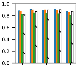
Pearson-r
