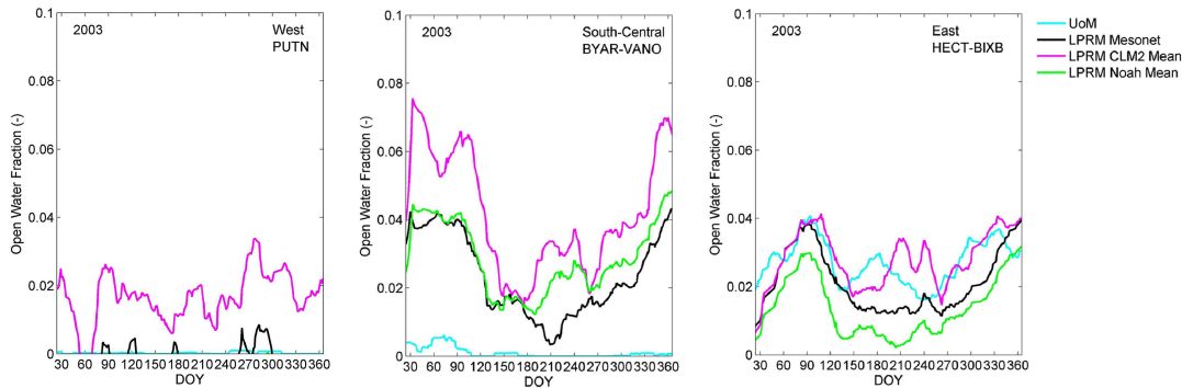
Fig. 1. Figure 5. Time series of the Open Water Fraction calculated with the LPRM, together with the OWFUoM, for the 0.25^\circ grids cells in the Western, South-Central and Eastern Oklahoma area (low pass filter)
