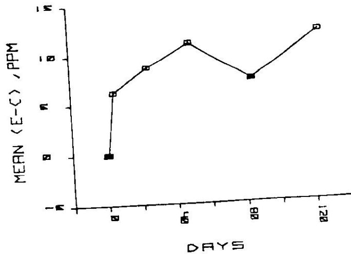
Figure 36. Mean net uptake of Zn between experimental and control, Thalassia roots and mangrove roots - Experiment II.
