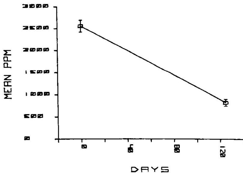
Figure 8. Mean net uptake of Cu between experimental and control, fouling organisms and sewage - Experiment I.
