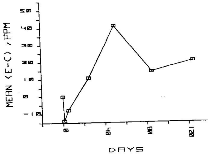
Figure 39. Mean net uptake of Cd and Cr between experimental and control, sea cucumber guts - Experiment II.
