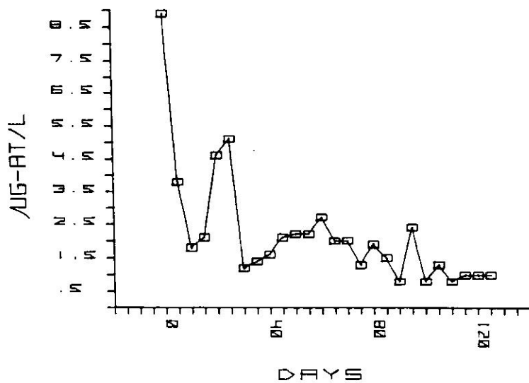
Figure 5. Dissolved reactive phosphate concentration Experiment I and II, experimental. Data points are mean values for 5 day period, excluding day 1.
