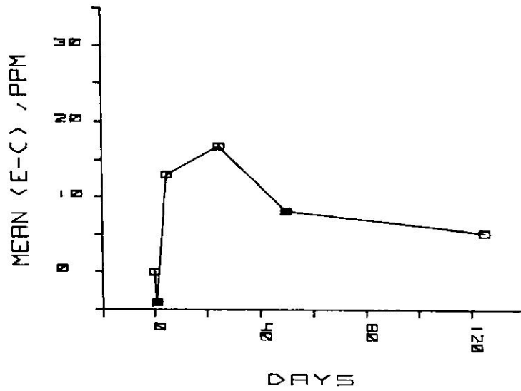
Figure 22. Mean net uptake of Ni between experimental and control, Thalassia leaves and urchin guts - Experiment I.
