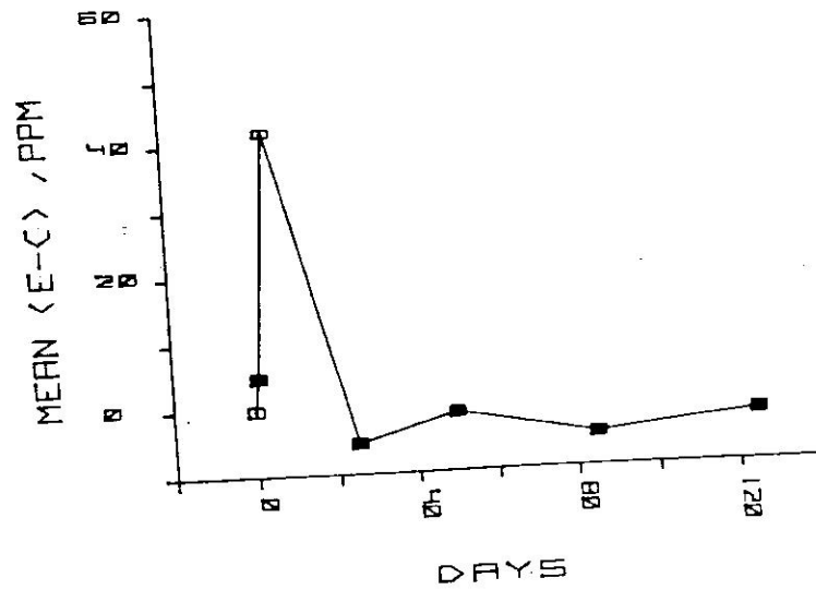
Figure 28. Mean net uptake of Ni between experimental and control, Thalassia roots and mangrove roots - Experiment II.
