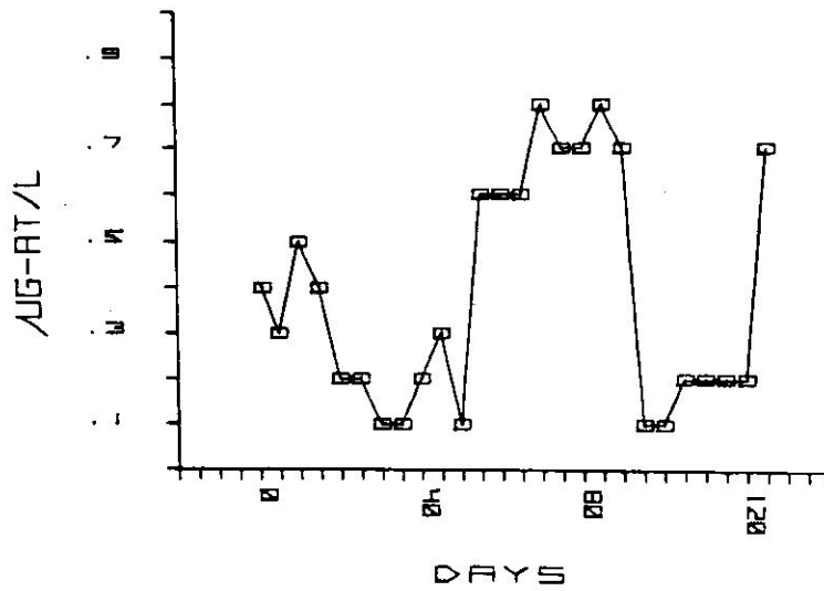
Figure 4. Dissolved reactive phosphate concentration Experiment I and II, control. Data points are mean values for 5 day period, excluding day 1.
