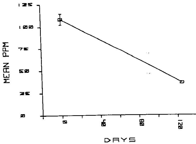
Figure 6. Mean net uptake of Cd between experimental and control, fouling organisms and sewage - Experiment I.
