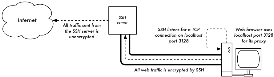
Figure 6.6: The SSH tunnel protects web traffic up to the SSH server itself.
