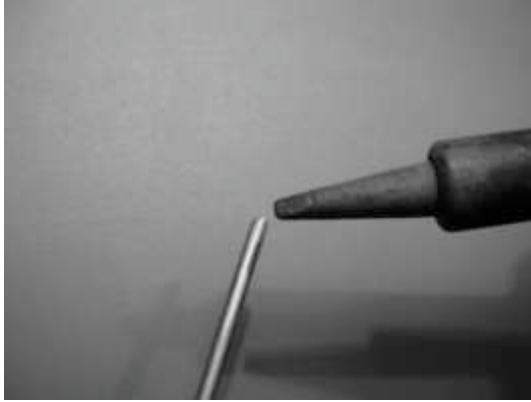
Figure 4.38: Tin the end of the wire before soldering.
